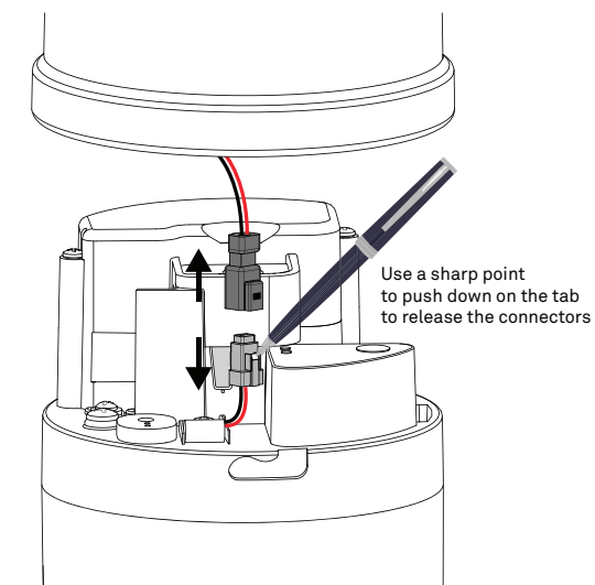
Figure 14 Disconnect pyranometer connector
