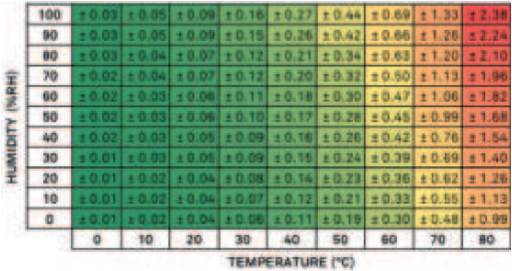
Figure 7 Vapor pressure sensor accuracy
