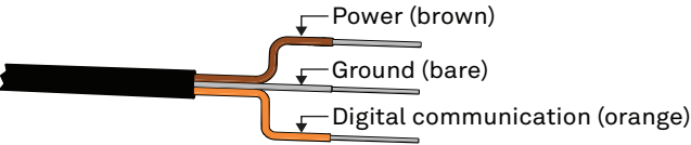
Figure 2 Pigtail wiring
