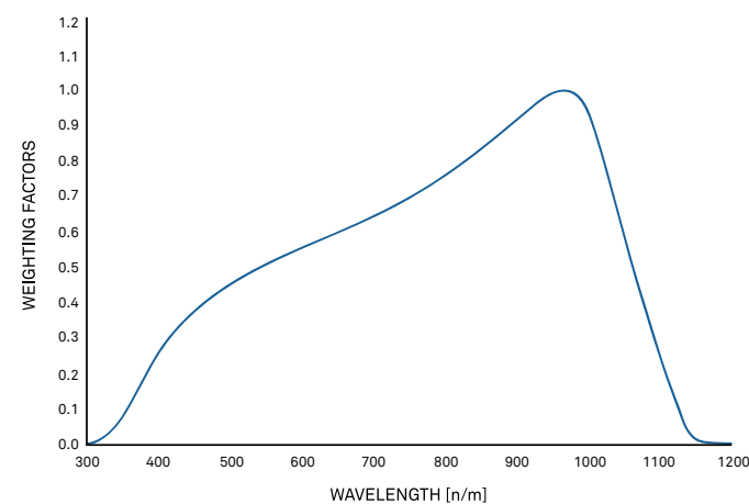
Figure 9 Spectral response estimate of Apogee silicon-cell pyranometers
