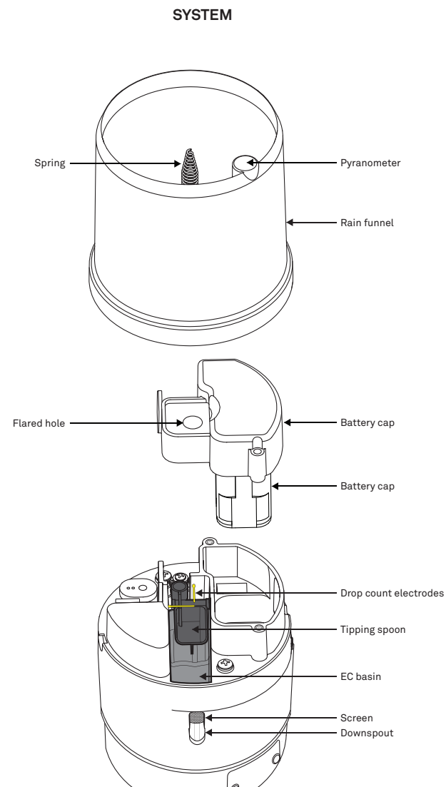
Figure 12 Rain funnel and rain gauge
