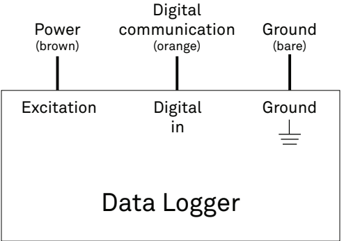
Figure 3 Three-wire SDI-12 wiring diagram
