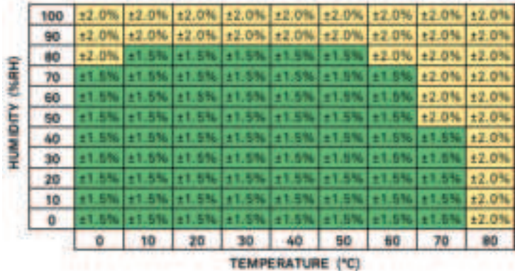
Figure 8 RH sensor accuracy
