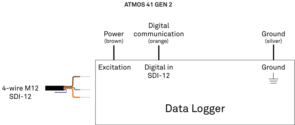
Figure 4 Four-wire M12 connector SDI-12 wiring diagram
