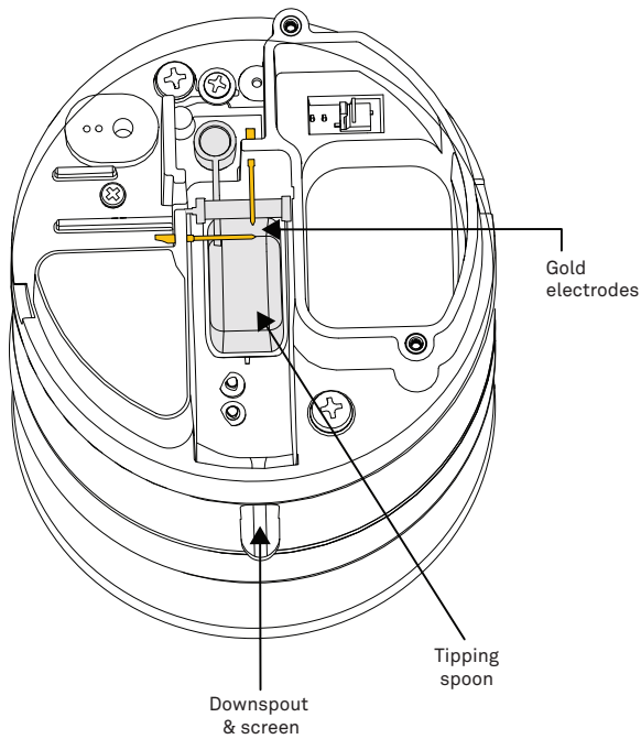
Figure 16 Downspout and screen
