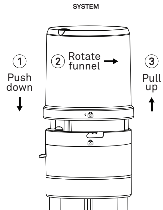
Figure 13 Removing ATMOS 41 Gen 2 rain funnel
