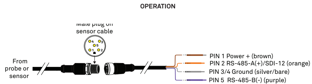
Figure 5 Four-wire M12 connector and pigtail adapter for use with screw terminals
