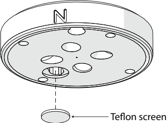
Figure 21 Teflon screen
