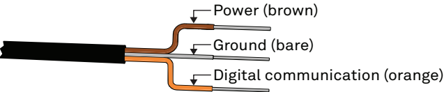
Figure 2 Pigtail wiring
