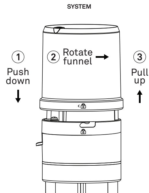
Figure 13 Removing ATMOS 41 Gen 2 rain funnel
