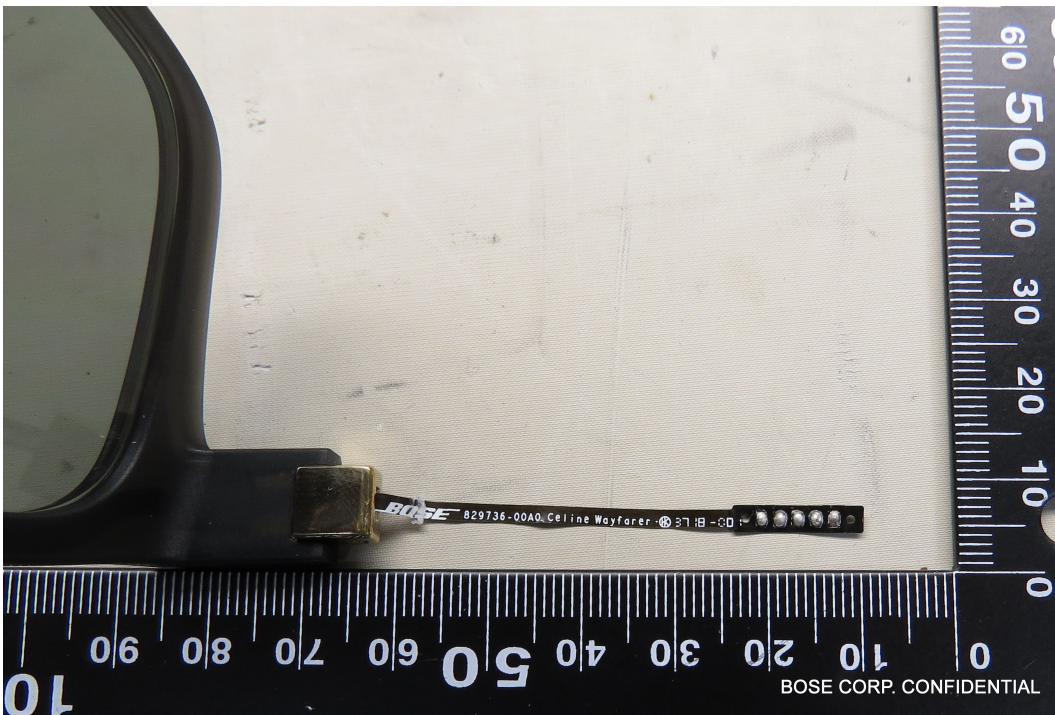
Left temple FFC connection (FFC is molded into the lens frame)
