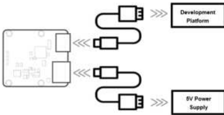
YDLIDAR GS2 AUXILIARY POWER SUPPLY
