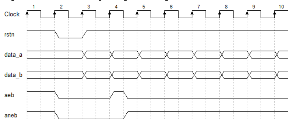
Figure 5-1 Gowin FP Comp IP Signal Timing
