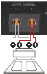
One subwoofer with a dual voice coil
