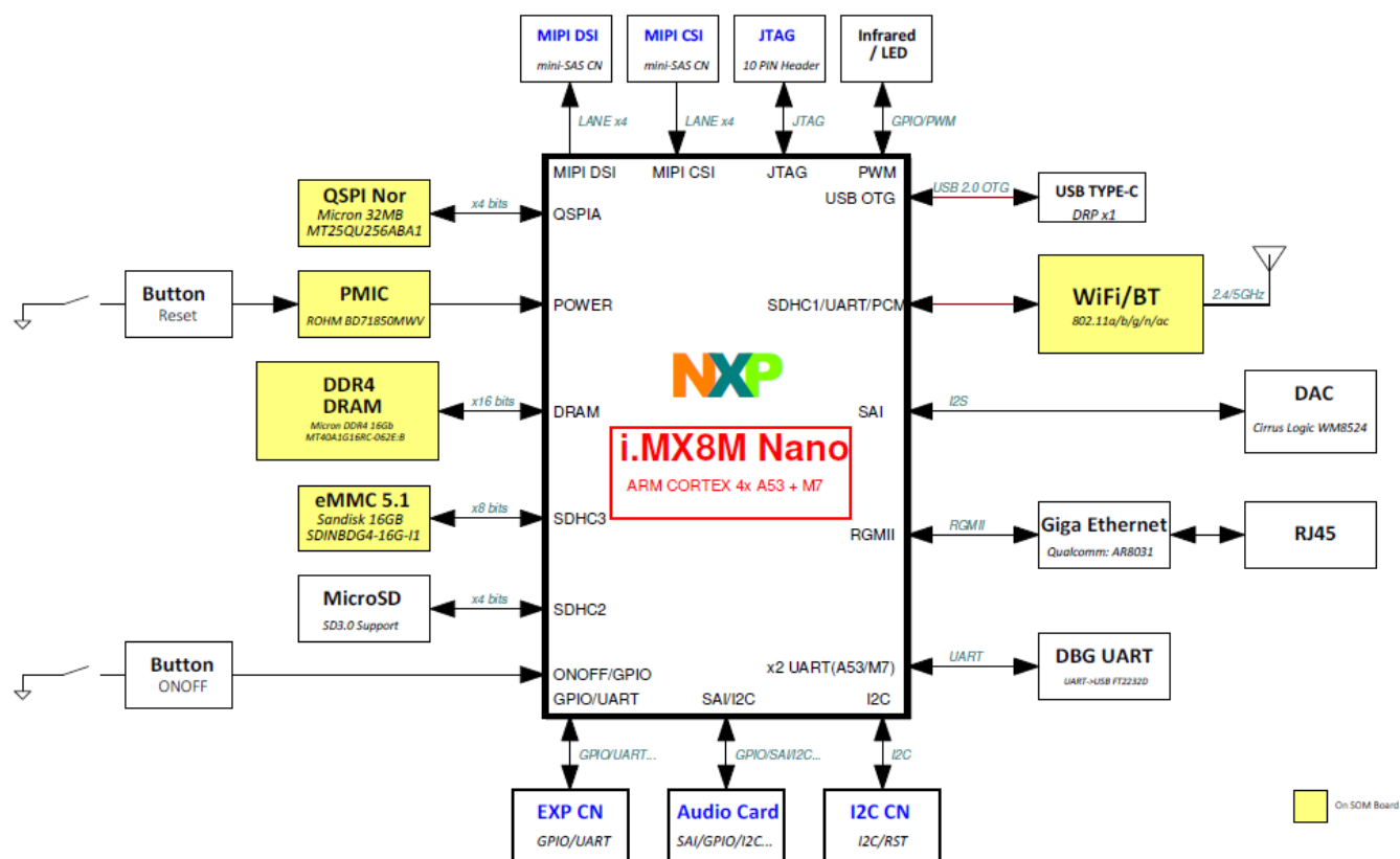
Figure 1. i.MX 8M Nano DDR4 EVK Block Diagram
