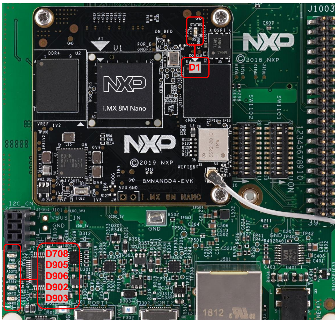
Figure 5. LED indicator
