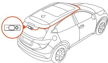
⑥ Installing the Rear Camera and Wiring
