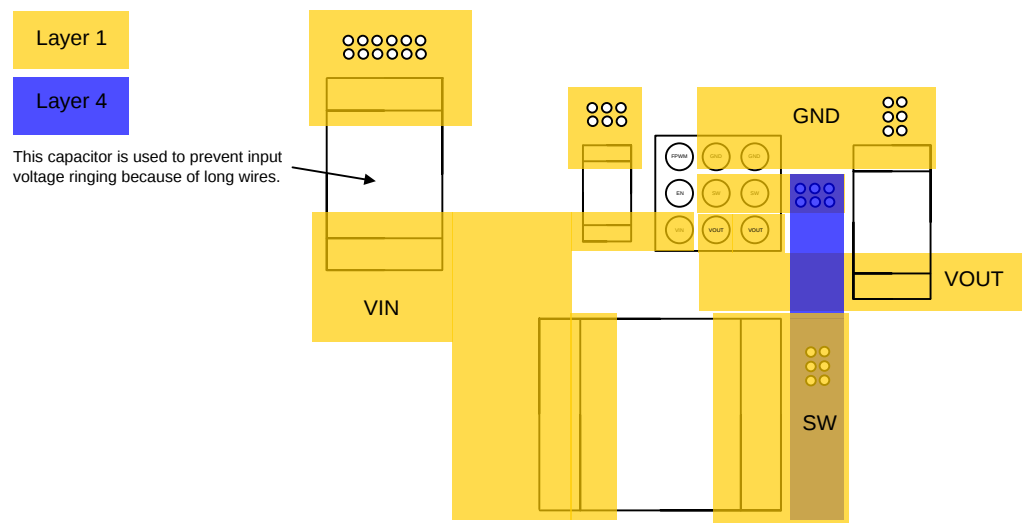
Figure 4. PCB Layout Guide
