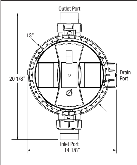
Figure 8. Dimensions, CS Cartridge Series Filter - Top View
