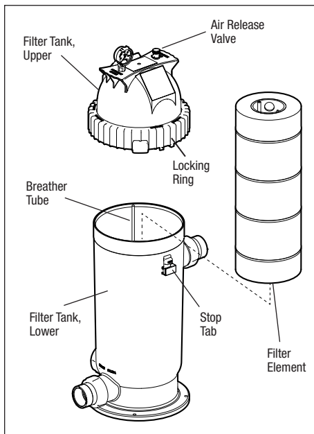
Figure 6. Filter Element Removal
