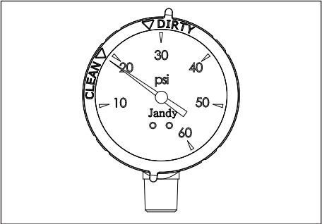
Figure 5. Pressure Gauge with Clean/Dirty Snap Ring
