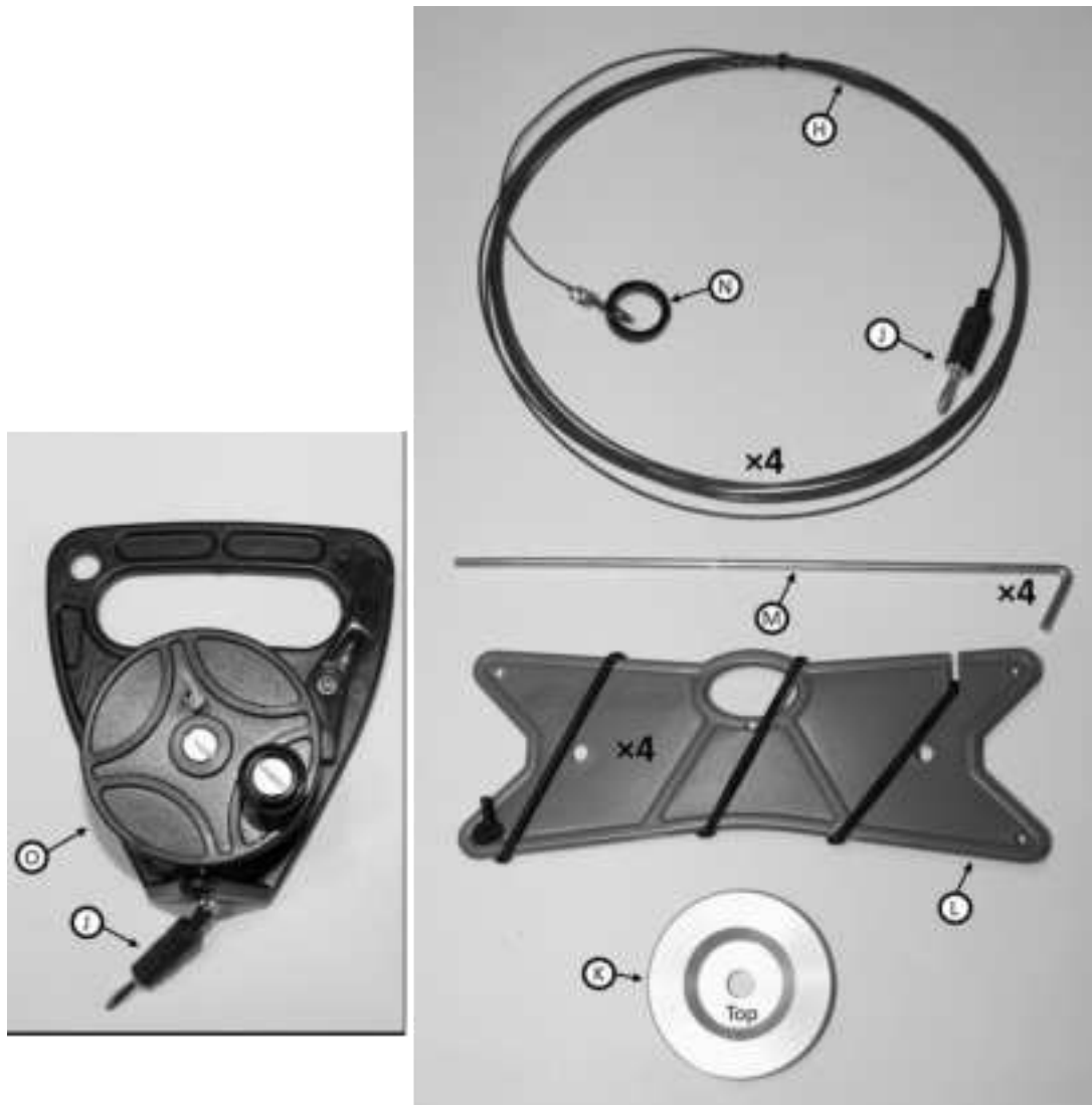
Plate 3. Counterpoise Components.
