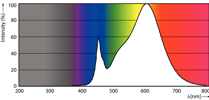
Spectral Power Distribution Colour - 13T8-6U/MAS/24-830/IF20/P/DIM 10/1
