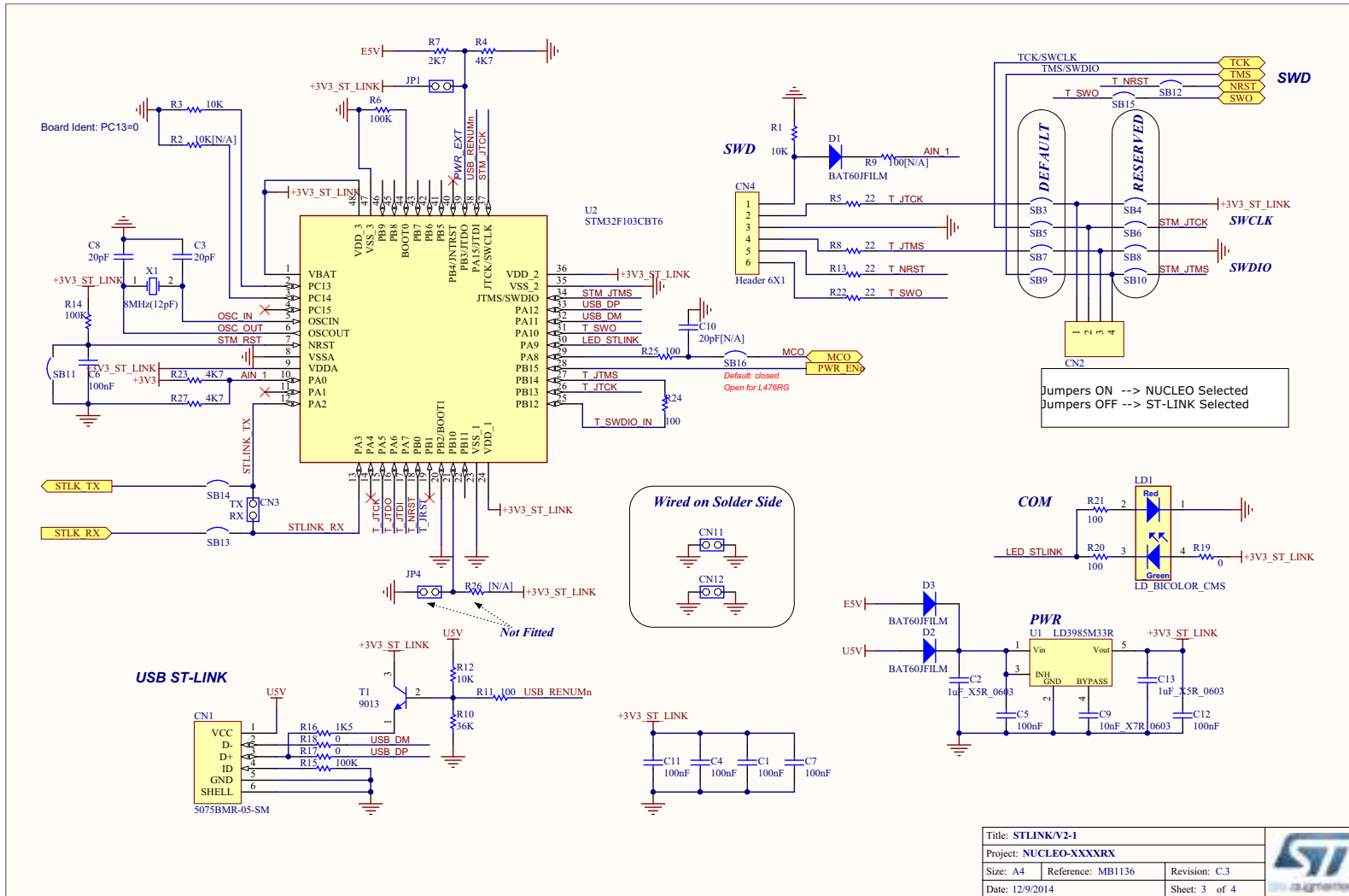
Figure 27. Electrical schematics (3/4)
