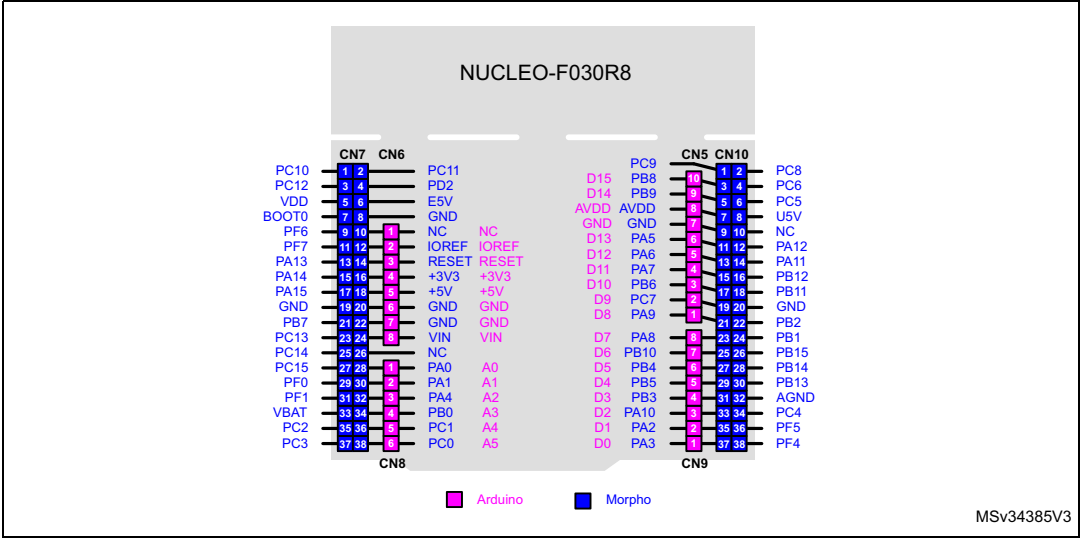
Figure 8. NUCLEO-F030R8
