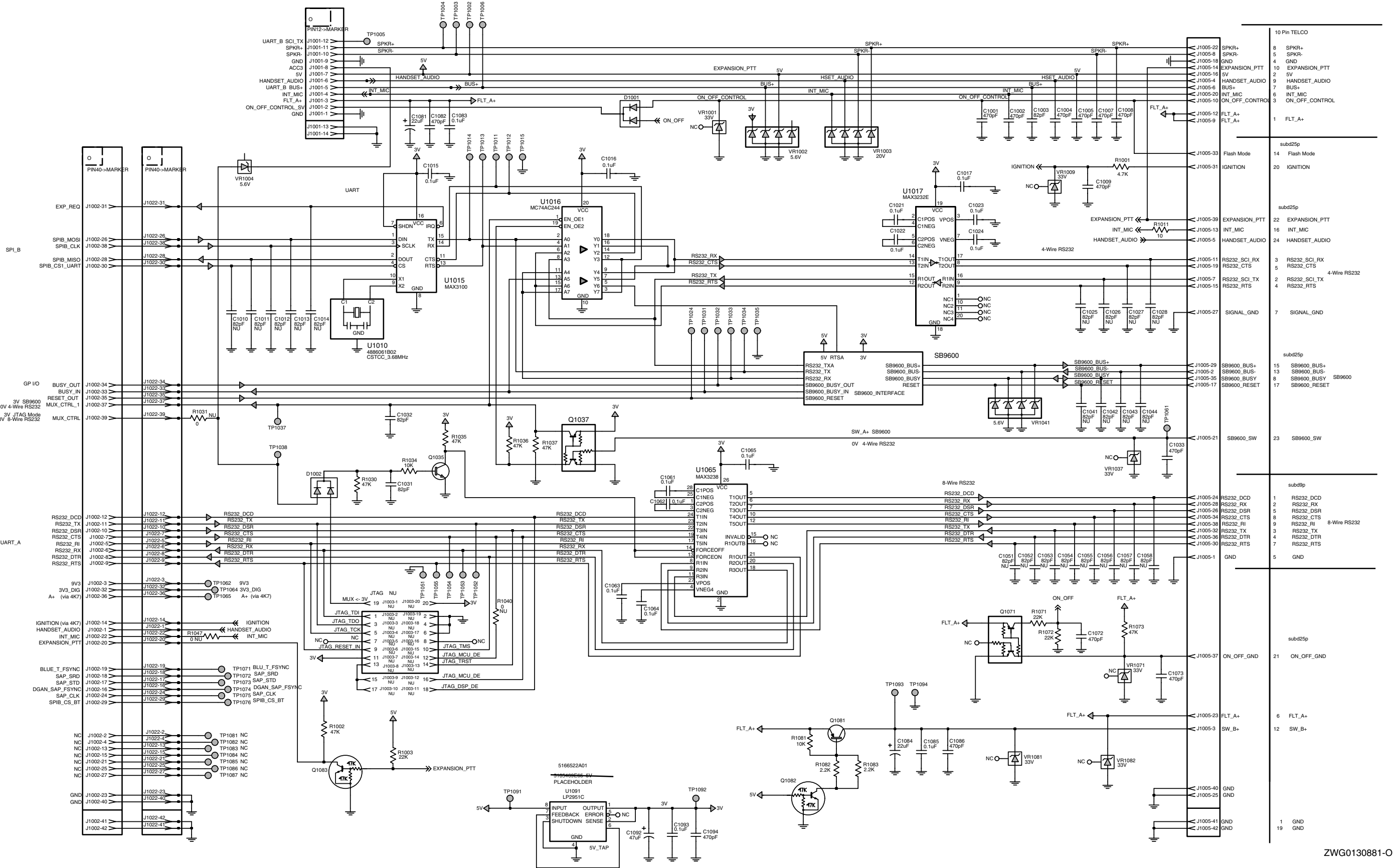
EXPANSION_HEAD / Expansion Board / Schematic Diagram
