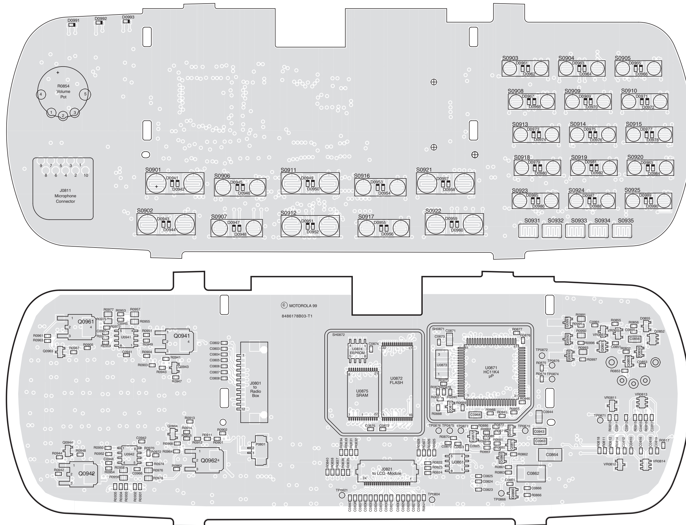
PCB / STANDARD_CONTROL_HEAD / BOTTOM &amp; TOP SIDE
