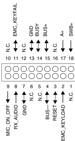
Figure 9 Pin Assignment of the Rear 18pin Connector of the Motorcycle Control Head
