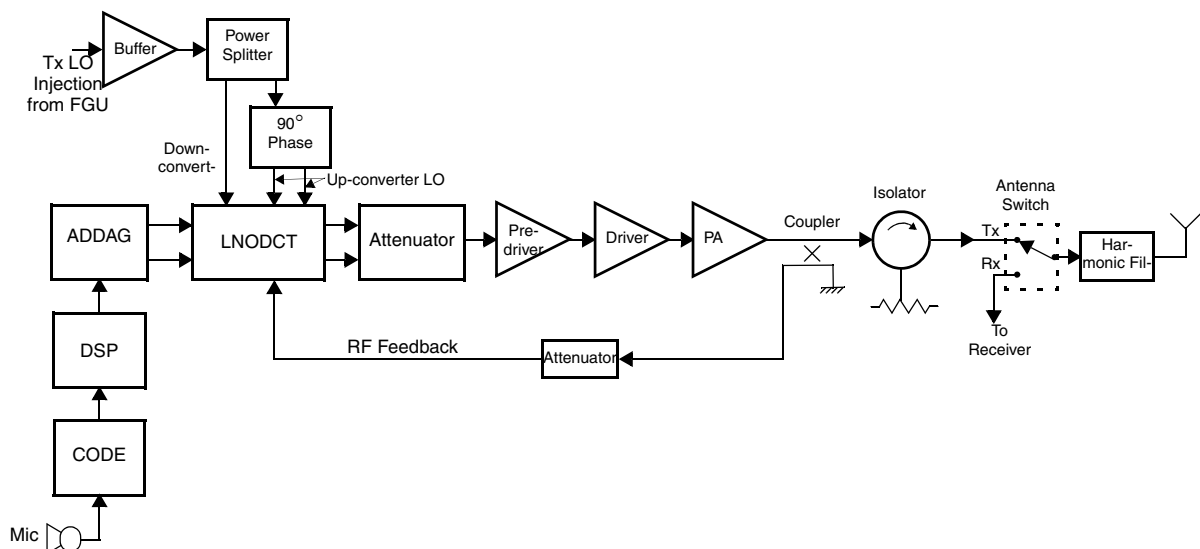
Figure 3 Transmitter Path Block Diagram
