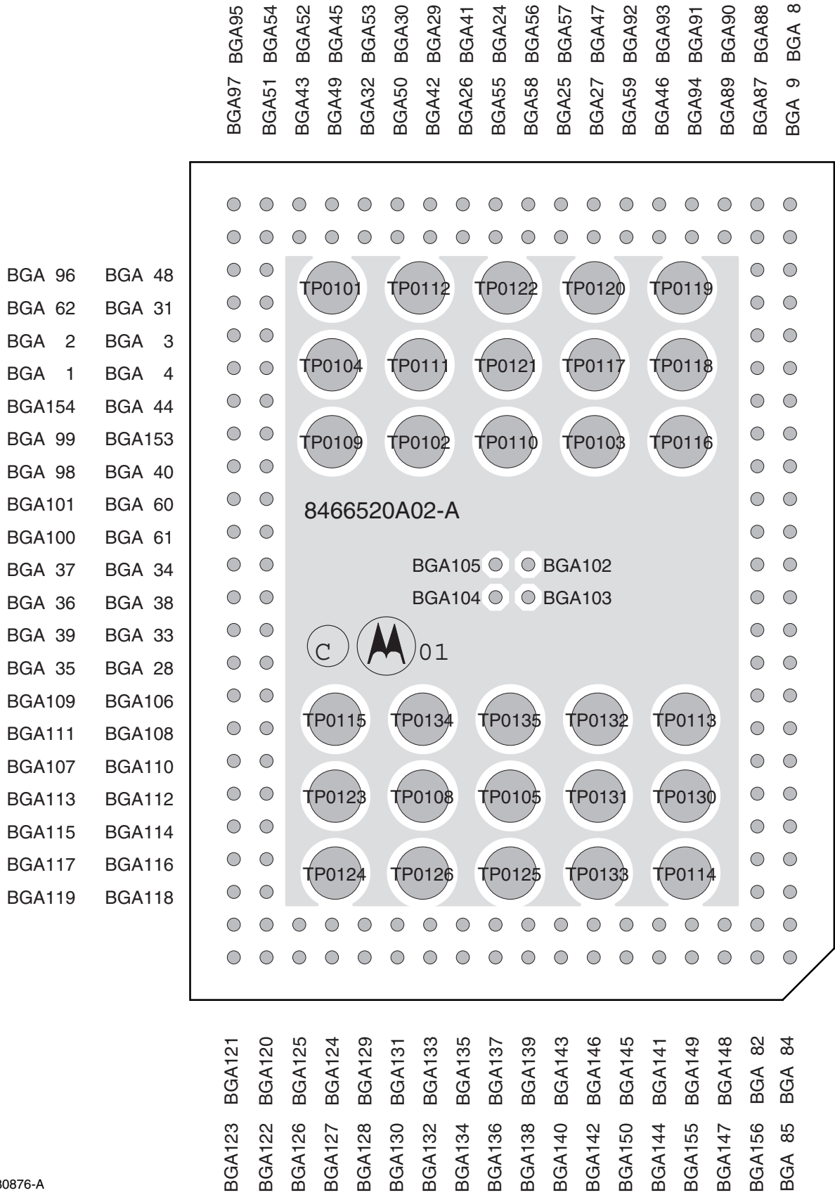
PCB / HDI_Controller 8466520A02_A / BOTTOM & TOP SIDE
