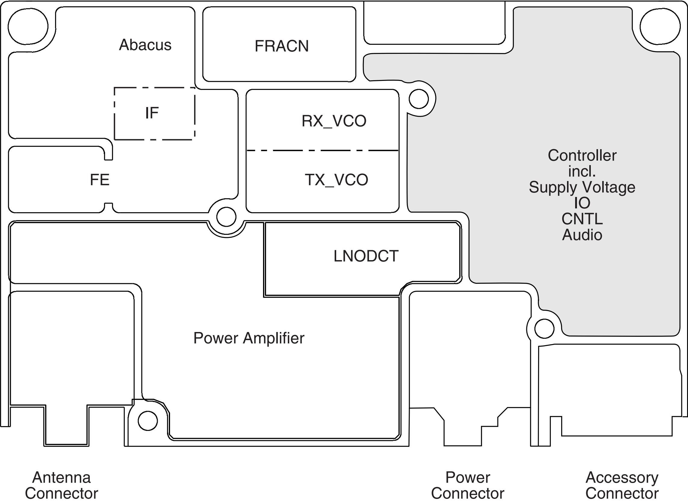
CHASSIS_OVERVIEW TRANSCEIVER
