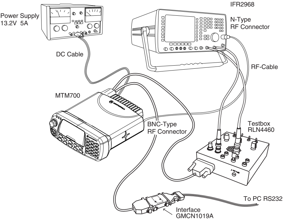
Figure 1 Troubleshooting Setup
