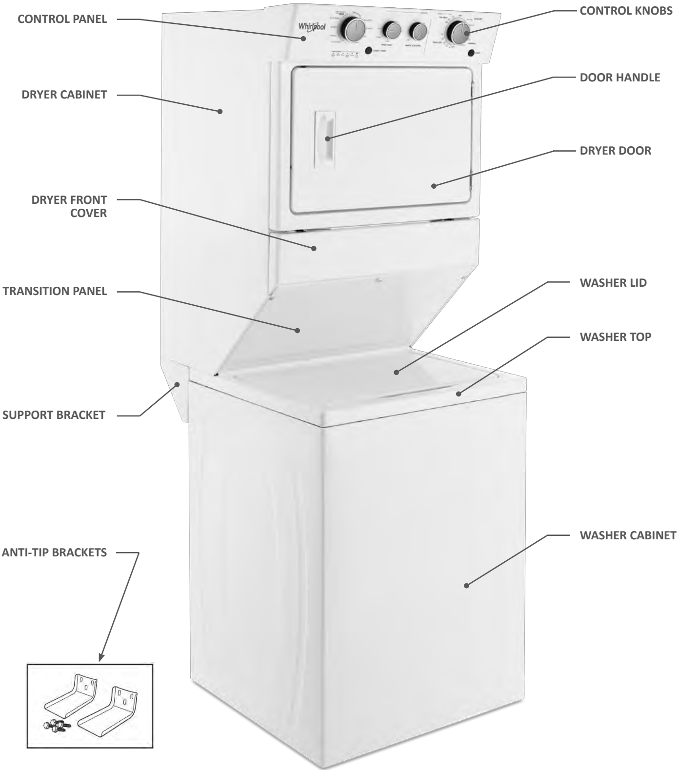
Figure 1 - 27" Stacked Laundry Center
