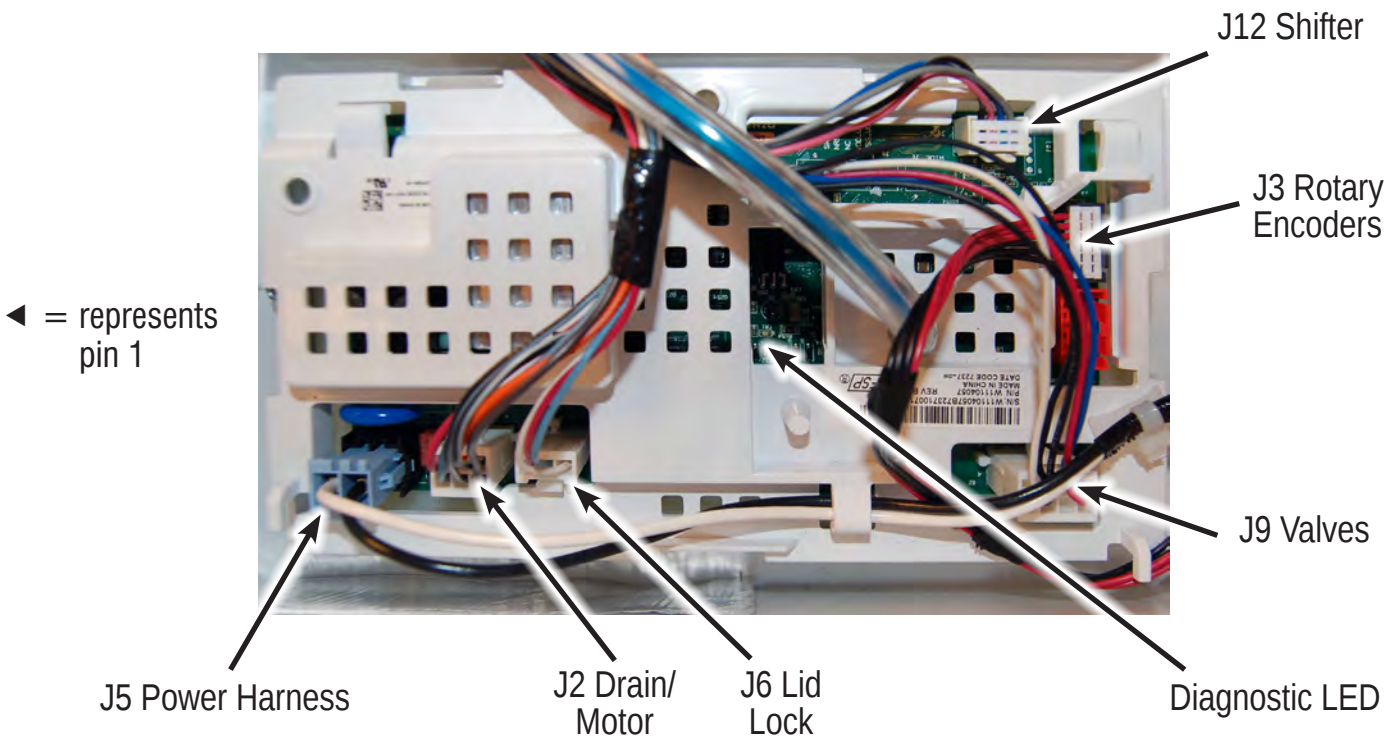
MAIN CONTROL BOARD (FIGURE 1)
