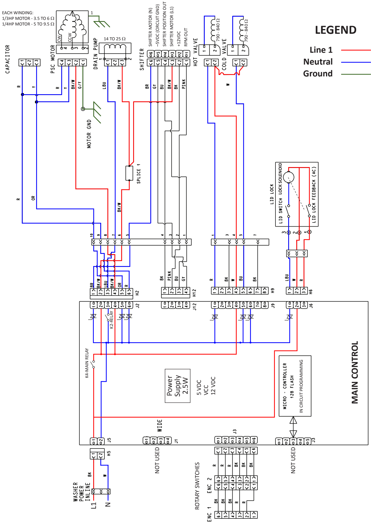
WIRING DIAGRAM
