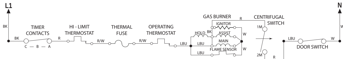
Figure 2 - Gas Dryer Heater Circuit
