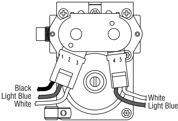
Figure 1 - Gas Valve
