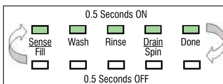
Figure 2 - Status LEDs flashing ON and OFF
