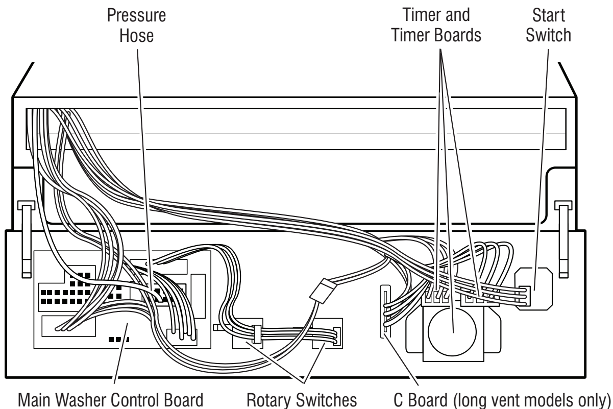
Figure 2 - Console Assembly Components
