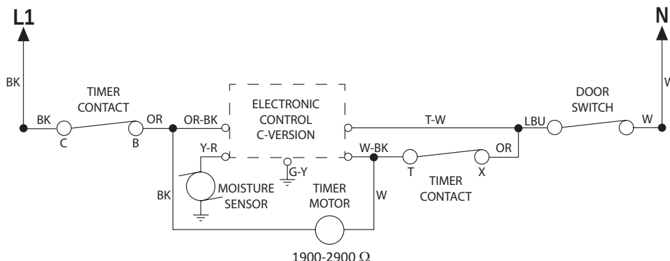
Figure 1 - Moisture Sensor Strip Circuit
