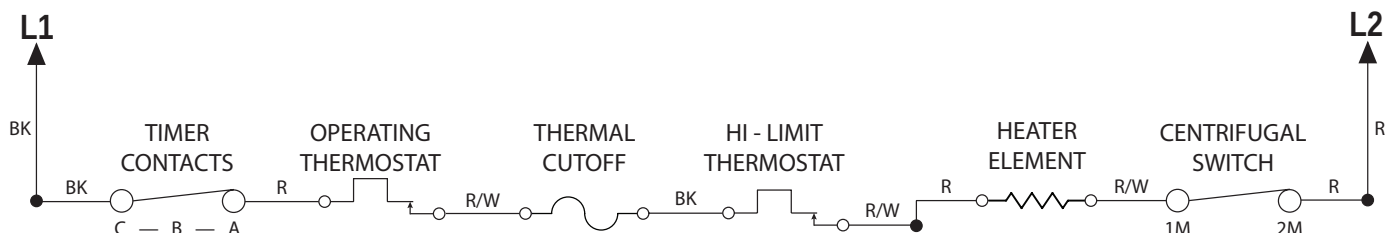
Figure 1 - Electric Dryer Strip Circuit
