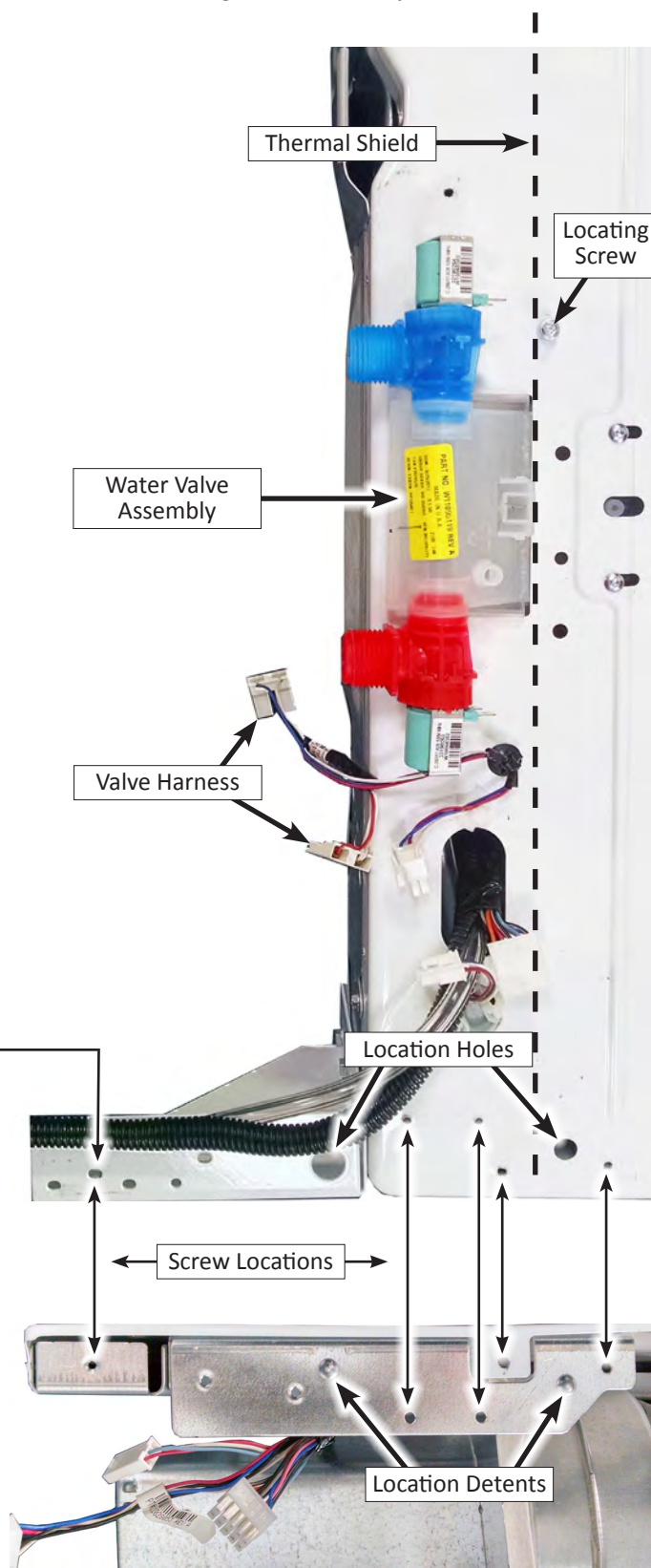
Figure 1 - Washer Top View
