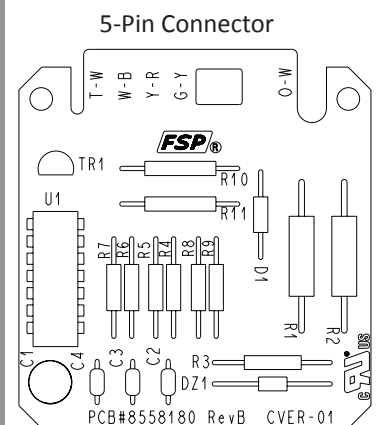
Figure 2 - Electronic Control Brd
