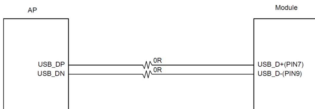
Figure 2-7 Reference circuit for USB 2.0 interface
