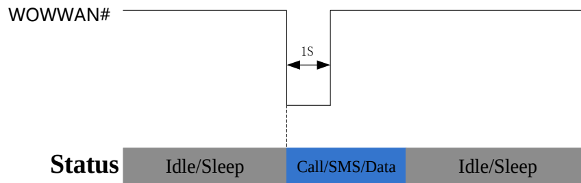
Figure 2-9 WOWWAN# timing
