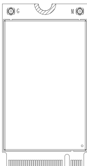
Figure 3-1 RF connectors
