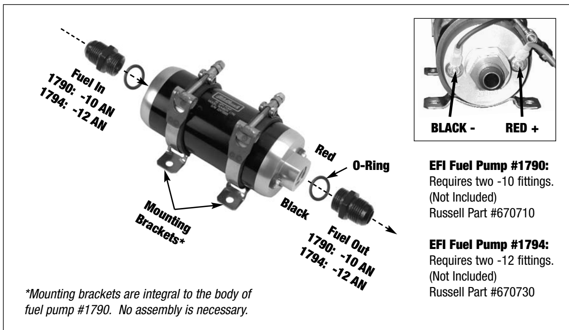
Figure 2 - Fuel Pump Fitting Assembly (1790 Shown)
