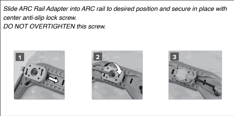
Figure 4 – ARC Rail Installation
