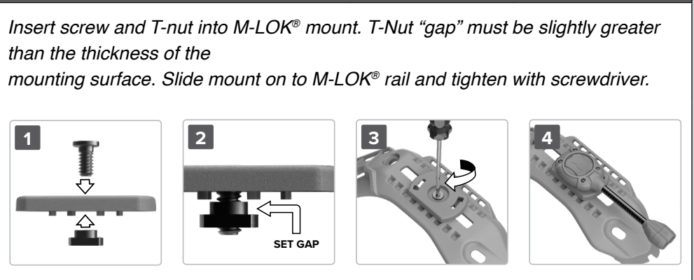
Figure 7 – MICH Mount Installation
