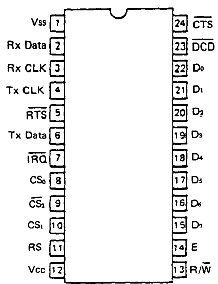
PIN CONFIGURATION
