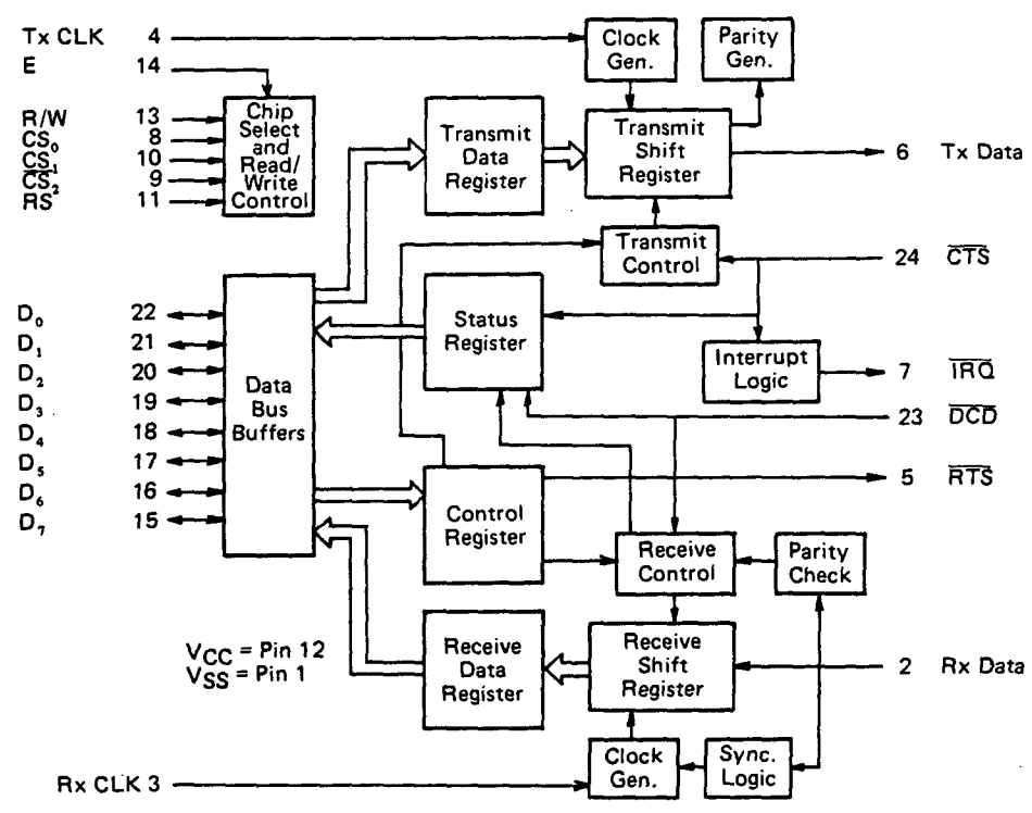
BLOCK DIAGRAM
