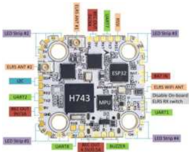
HDZero Halo FC – Top View (MPU6000)
