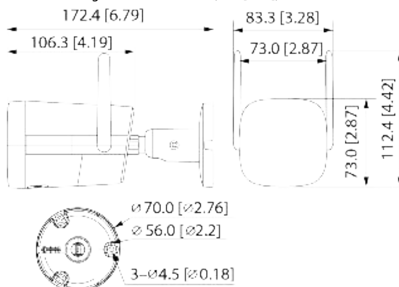
Figure 4-2 Dimensions (mm [inch])
