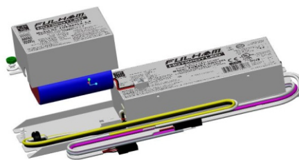
Exploded View
