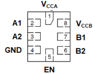
Figure 5. UQFN8
