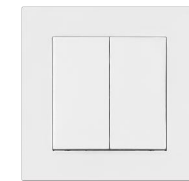
SR-MT2835KAC-NK4-SW 4 Push buttons, 2 Channels, Output current 2*5.1A Max. 2*390W LED load, 2*1170W incandescent, HV halogen loads
