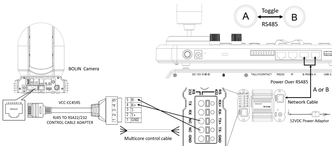
RS485 Connection – Via Junction Box - Camera with RS422 RJ45 to Phoenix adapter
