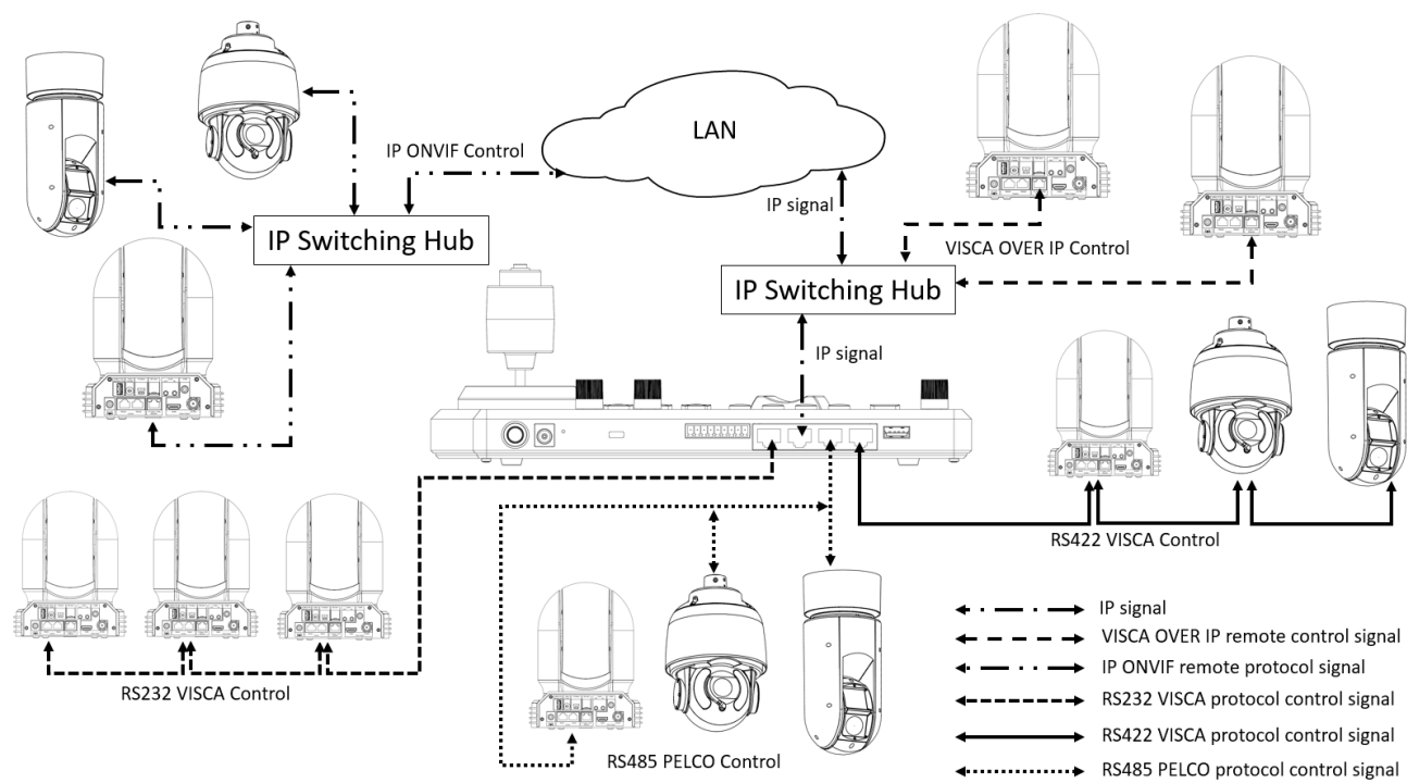
Cross-Protocol Mix Control - Using VISCA, PECLO, VISCA OVER IP, ONVIF IP Control Protocol in one single system.
