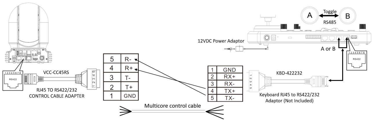
RS485 Connection - Use RJ45-RS422 Phoenix adapter - Camera with RS422 RJ45 connector
