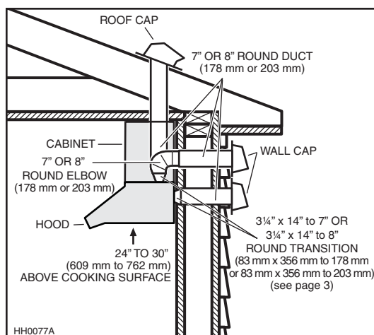
UP27I (DUAL INTERIOR BLOWER) TYPICAL ROUND DUCTWORK
