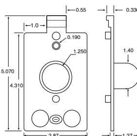
SS3-AB & SS3-ABN Domed Mounted Bracket
