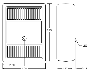
GENERAL DIMENSIONS
