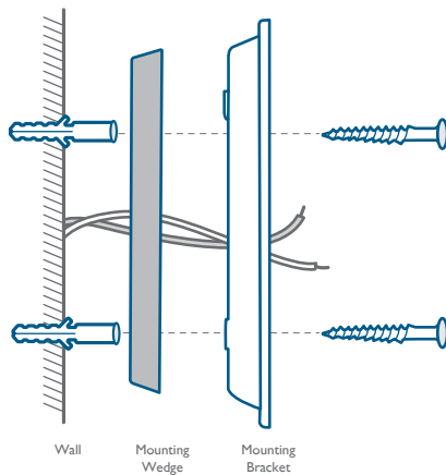
With 15° Mounting Wedge
