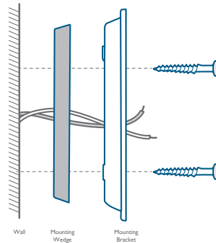
With 15° Mounting Wedge
