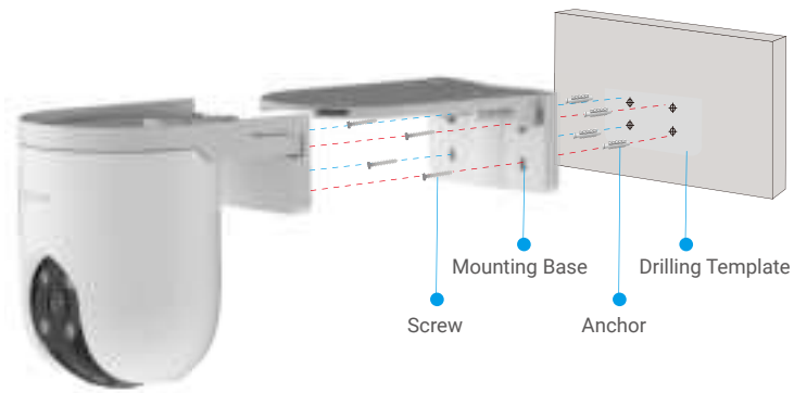
Fig. 2 Wall Mount
