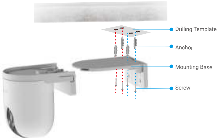
Fig. 1 Ceiling Mount
