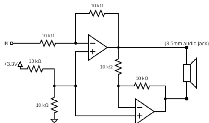
Figure 5. Audio out
