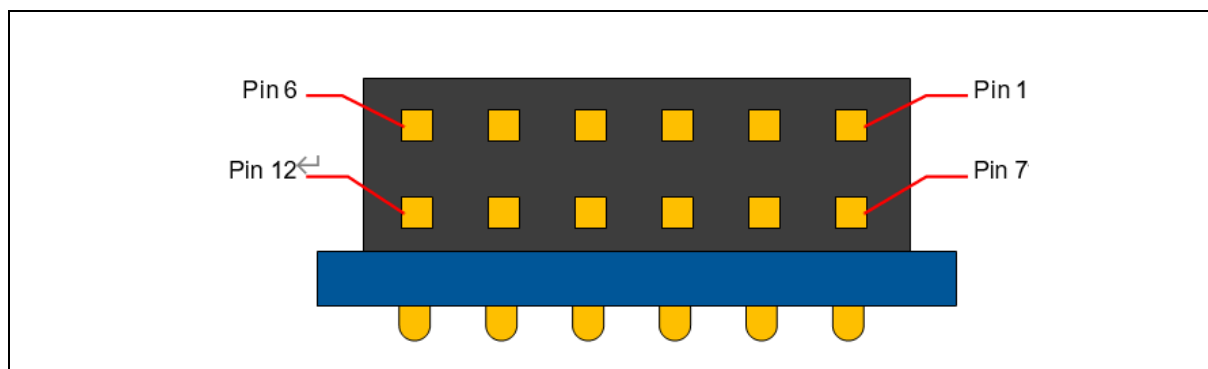
Figure 4. PMOD connector
