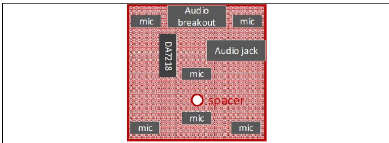
Figure 7. MIC-Board view
