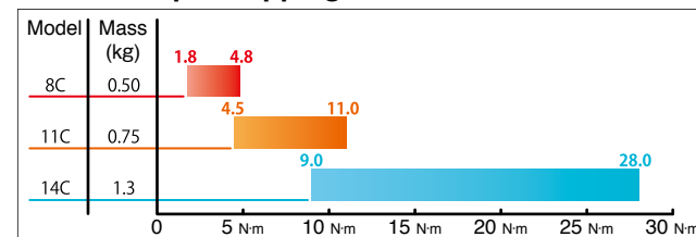
■ Max. Torque Mapping
