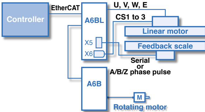
[Typical system configuration] For linear motor
