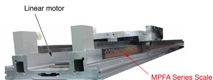
Linear motor drive stage with position feedback of MPFA Series Scale
