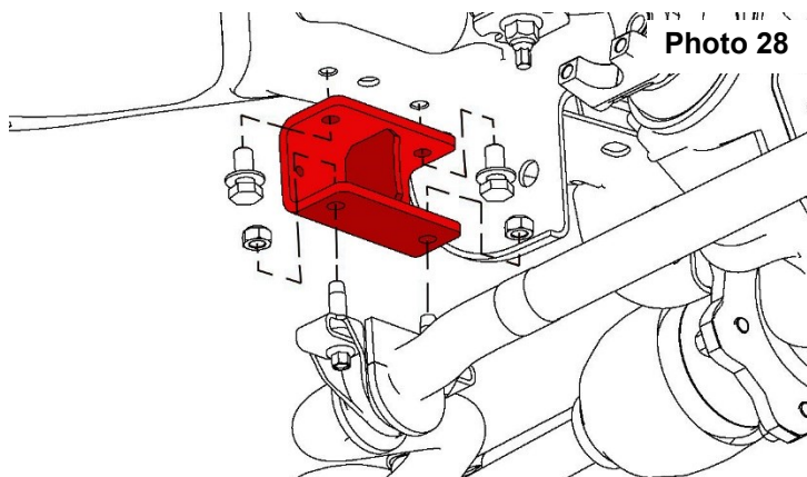
Install sway bar drop bracket.
