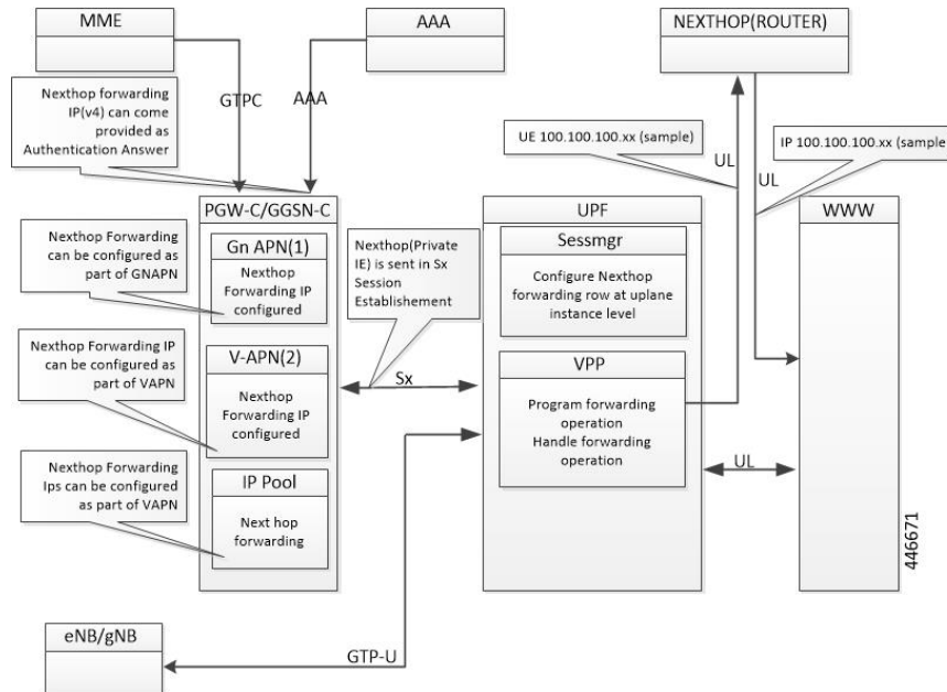
Figure 29: Nexthop Forwarding
