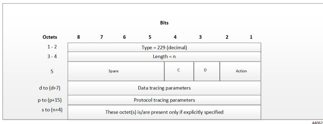
Figure 12: Subscriber Tracing
