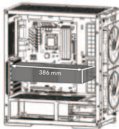
GPU Length Clearance
