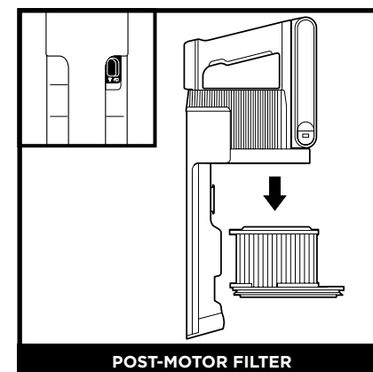
POST-MOTOR FILTER
