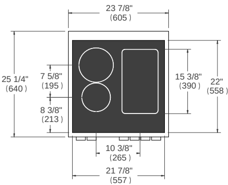
WORKTOP DETAILS
