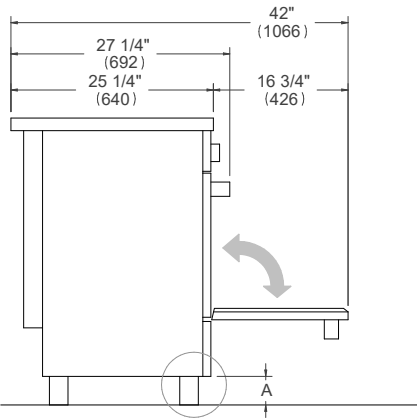
WORKTOP DETAILS
