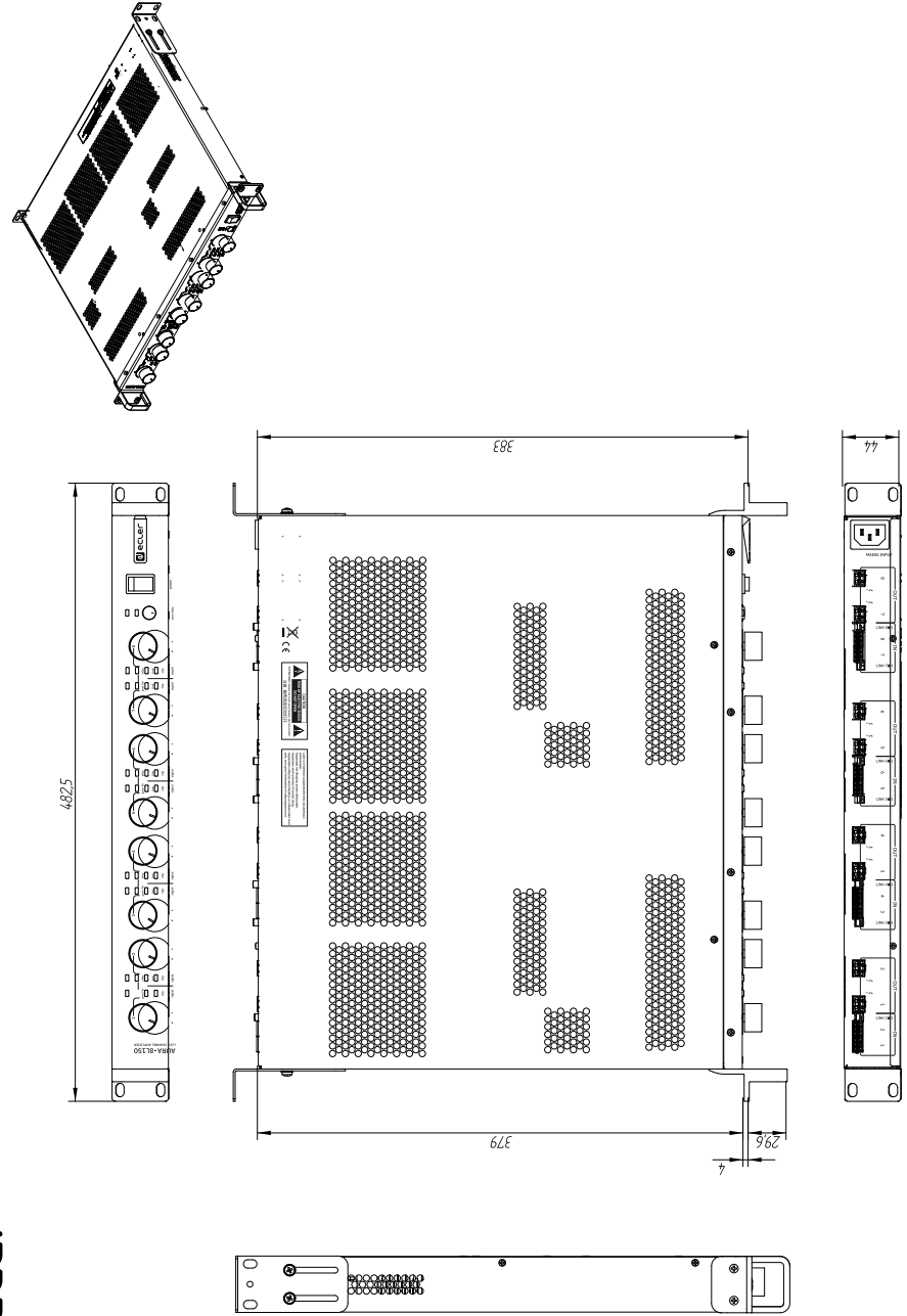
Ecler AURA-8L150 Mechanical Diagram
