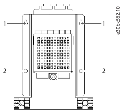
Illustration 5: Mounting Holes of the Assembly Plate
