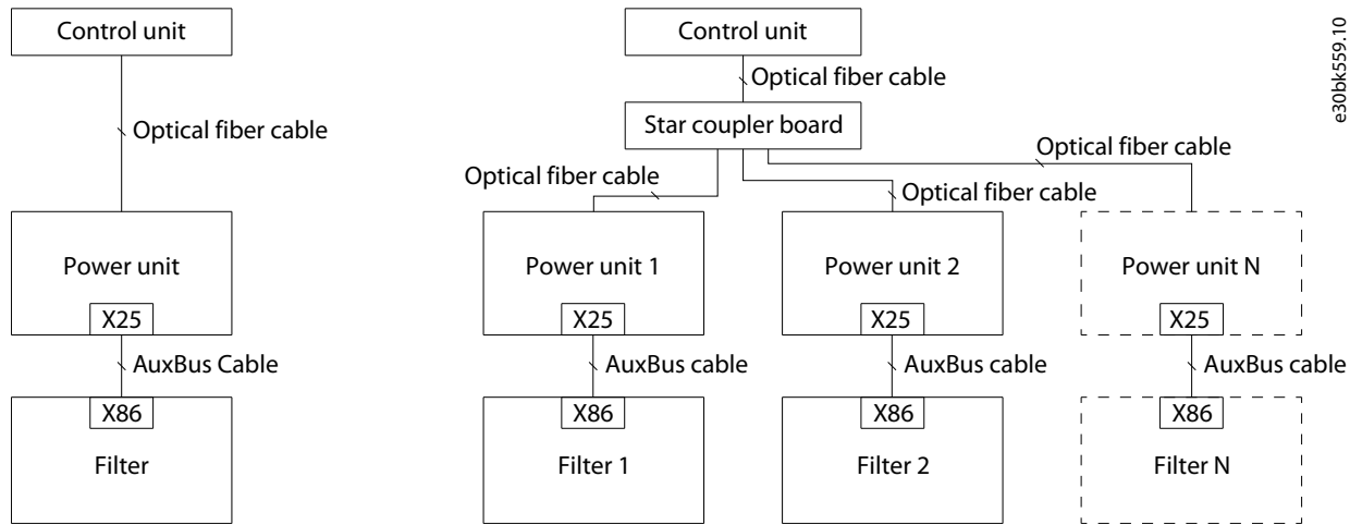
Illustration 14: AuxBus Topology
