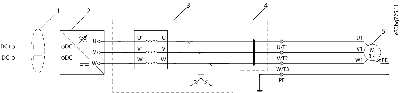
Illustration 16: Wiring Diagram for Inverter and dU/dt Filter
