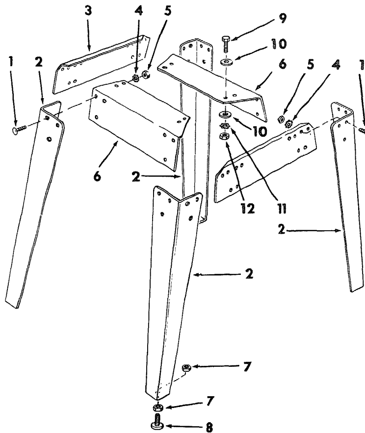
FIGURE 7 - LEGS
