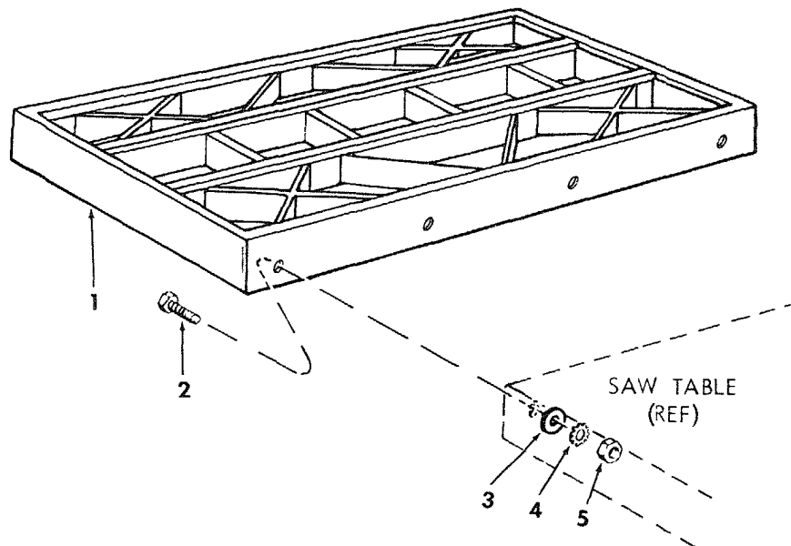
FIGURE 6 - TABLE EXTENSIONS
