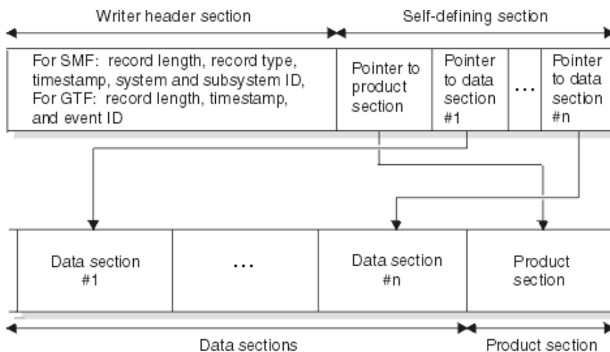
Figure 57. General format of trace records written by Db2
