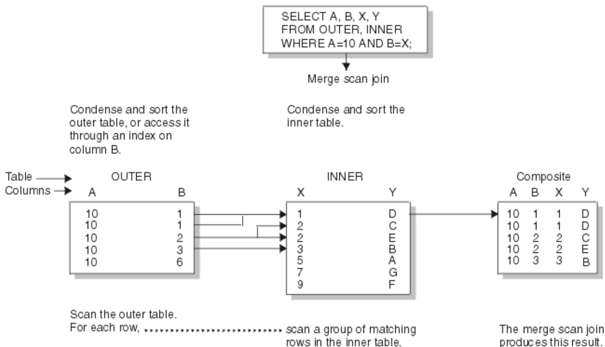
Figure 50. Merge scan join
