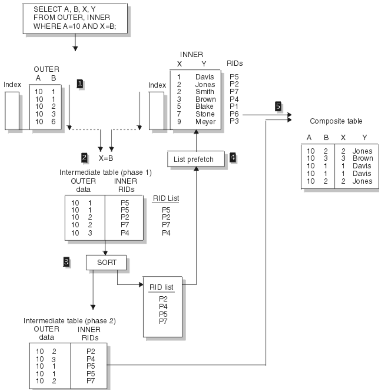
Figure 51. Hybrid join (SORTN_JOIN='Y')
