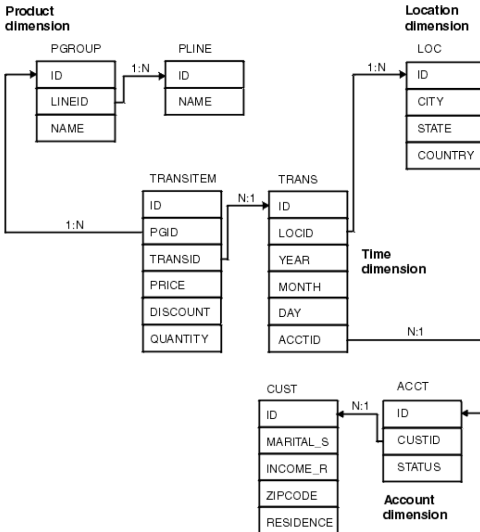
Figure 13. Multi-fact star schema
