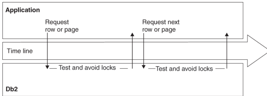
Figure 18. Best case of avoiding locks by using the ISOLATION(CS) and CURRENTDATA(NO) options
