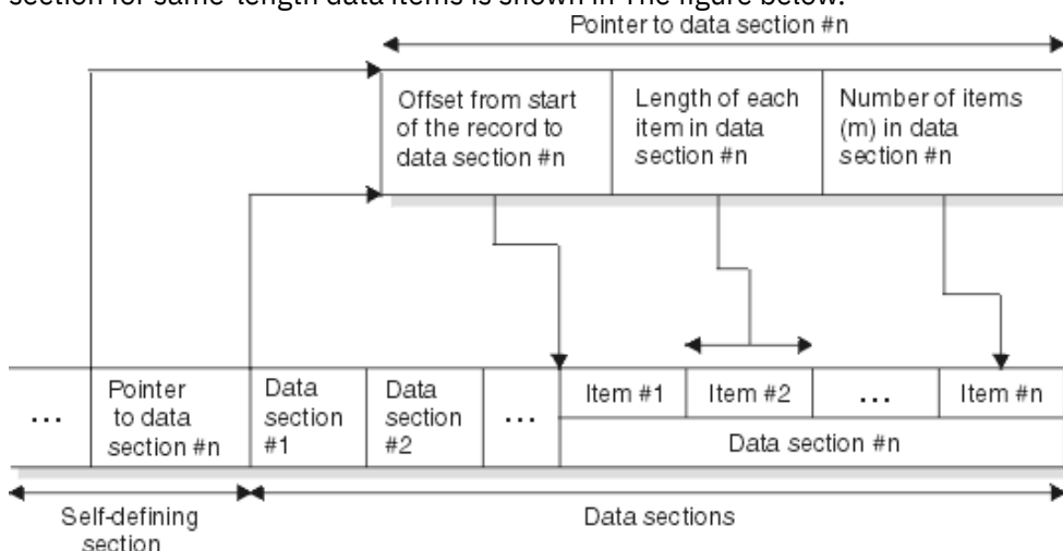
Figure 62. Relationship between self-defining section and data sections for same-length data items
