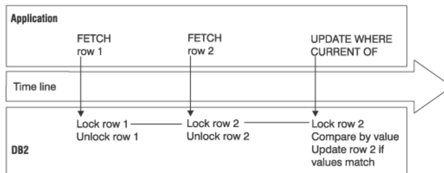
Figure 15. Positioned updates and deletes with a static sensitive scrollable cursor and with optimistic concurrency control
