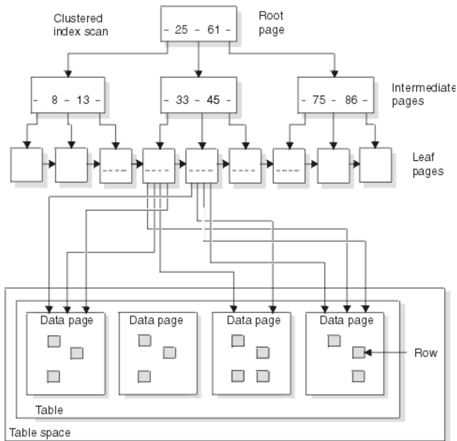
Figure 33. A nonclustered index scan
