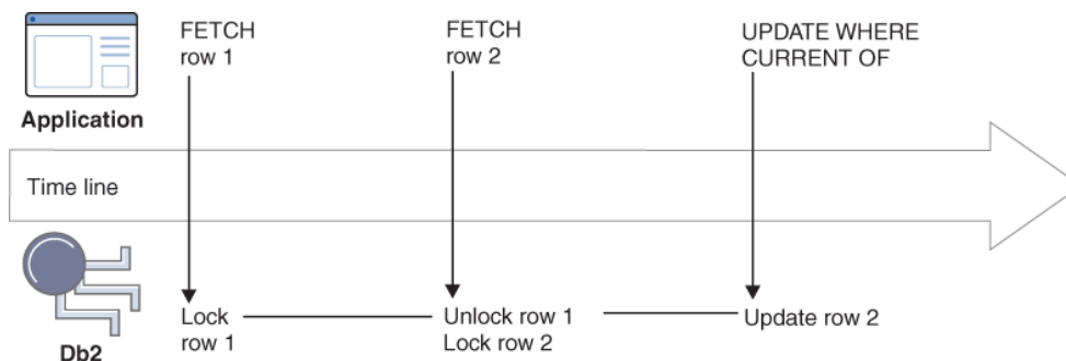
Figure 14. Positioned updates and deletes with a static non-scrollable cursor and without optimistic concurrency control
