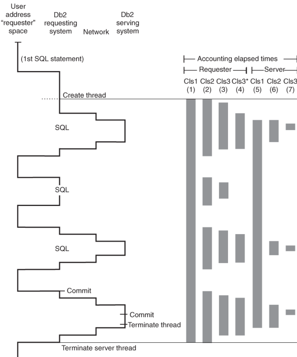
Figure 43. Elapsed times in a DDF environment as reported by Tivoli OMEGAMON XE for Db2 Performance Expert on z/OS
