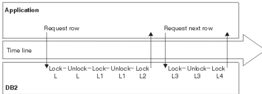
Figure 16. How an application that uses RS isolation acquires locks when no lock avoidance techniques are used
