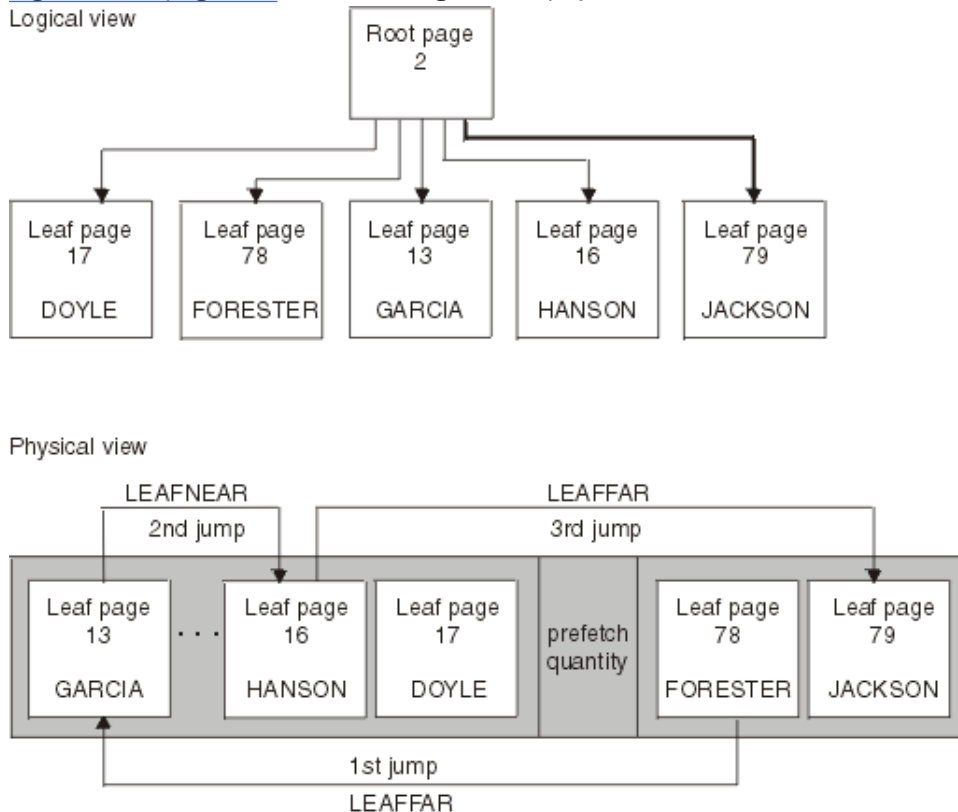
Figure 30. Logical and physical views of an index in which LEAFNEAR=1 and LEAFFAR=2
