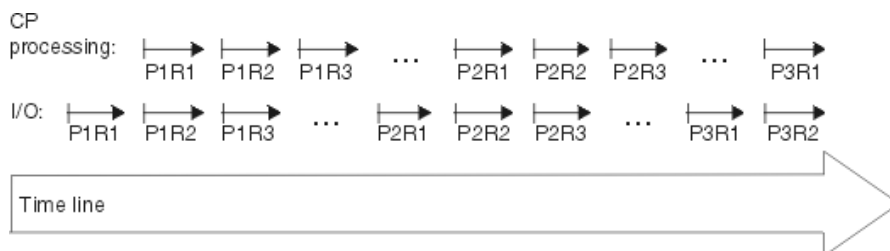
Figure 20. CP and I/O processing techniques
