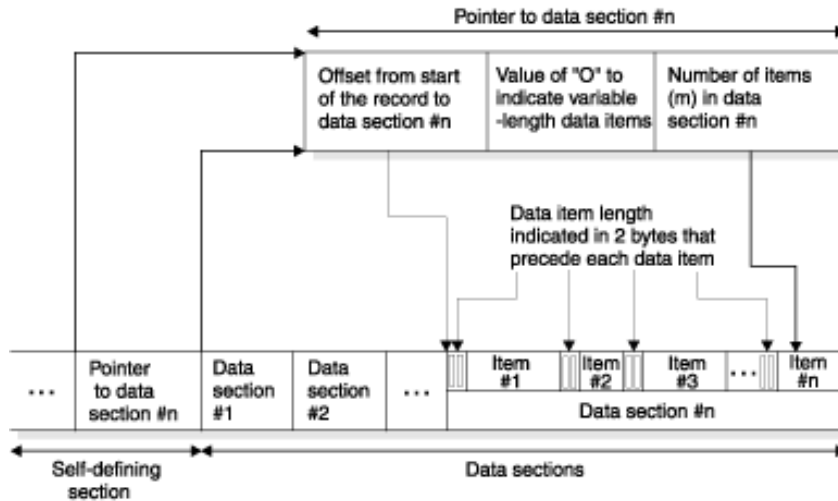
Figure 63. Relationship between self-defining section and data sections for variable-length data items
