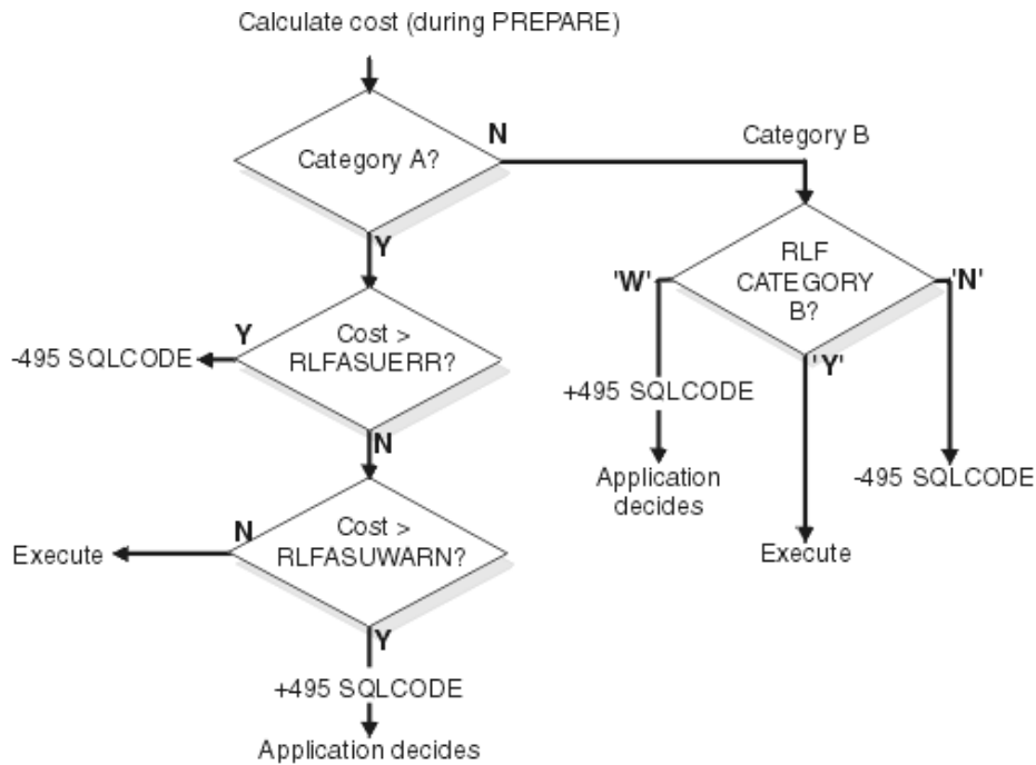
Figure 8. Processing for predictive governing
