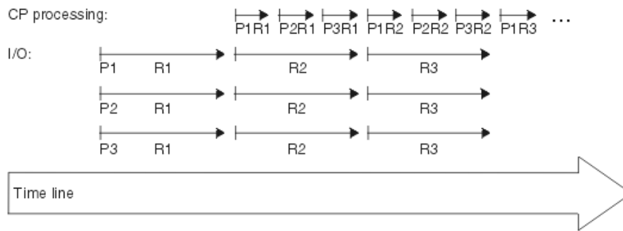
Figure 21. CP and I/O processing techniques
