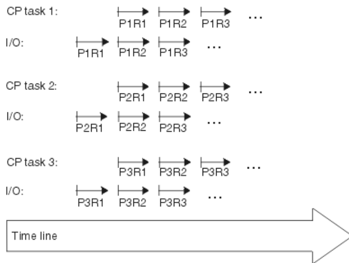
Figure 22. CP and I/O processing techniques
