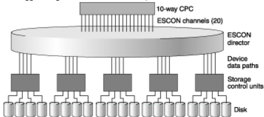
Figure 23. I/O configuration that maximizes performance for an I/O-intensive query
