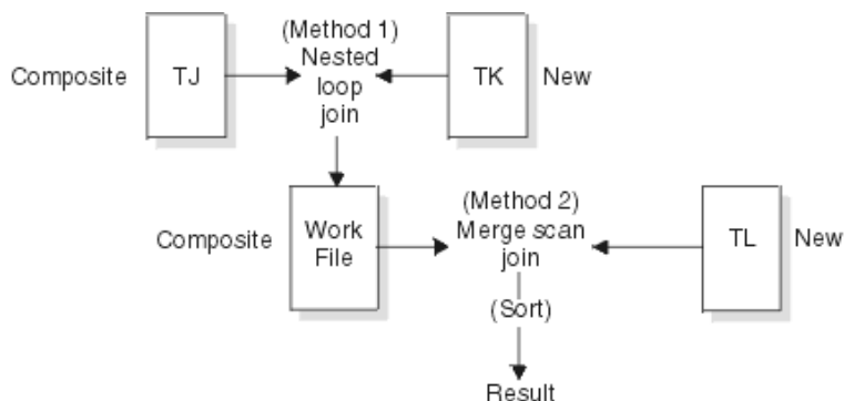
Figure 48. Two-step join operation
