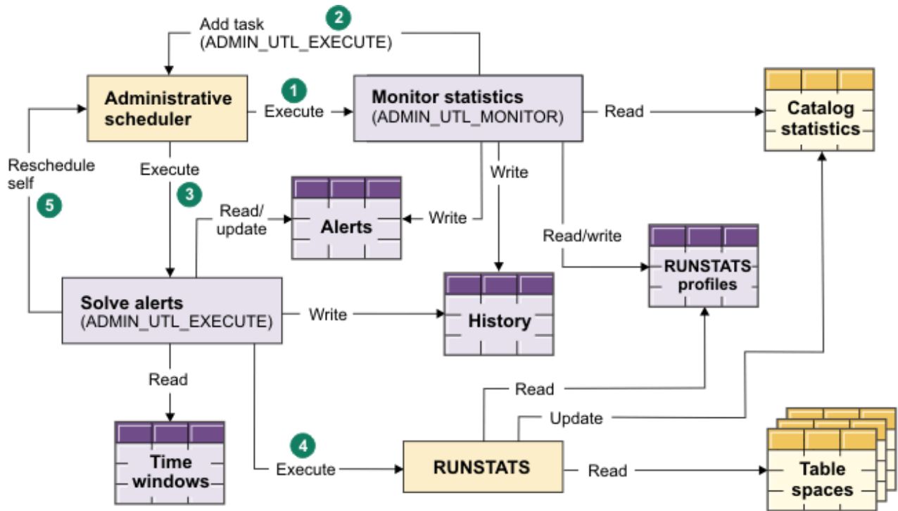
Figure 31. Object interactions for autonomic statistics maintenance in Db2
