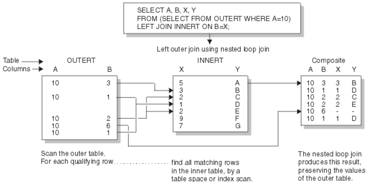
Figure 49. Nested loop join for a left outer join
