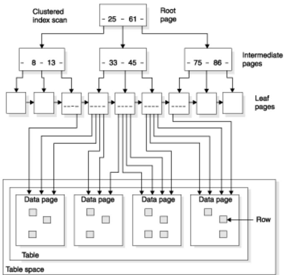
Figure 32. A clustered index scan
