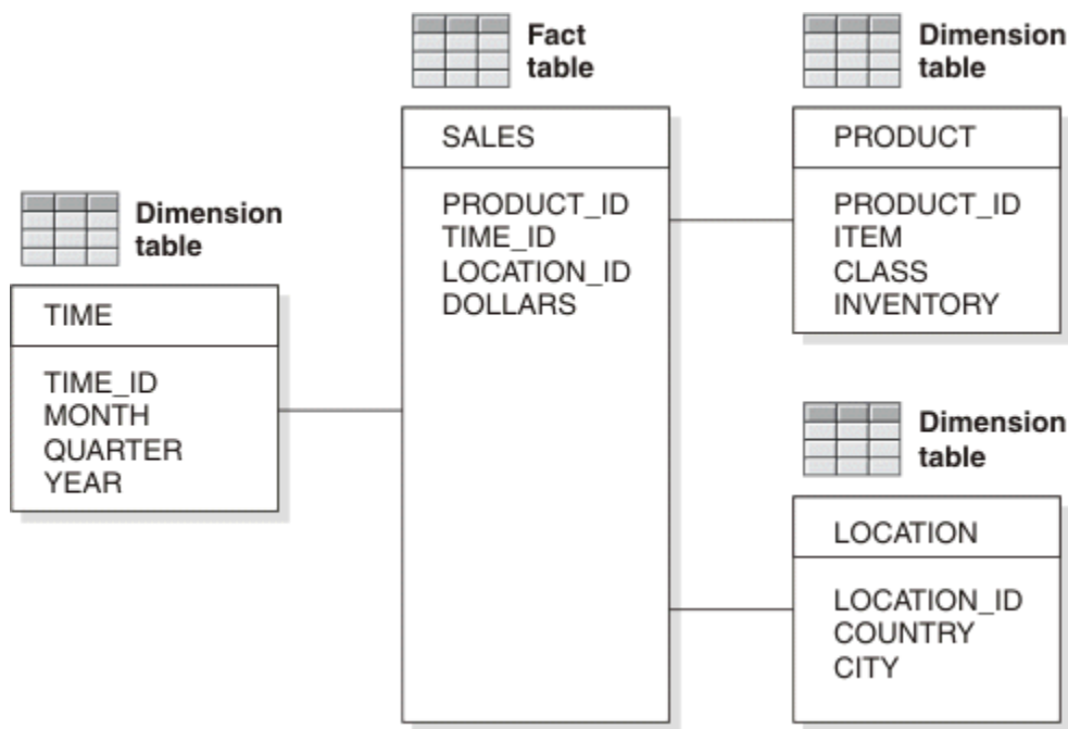
Figure 53. Example star schema with three dimension tables
