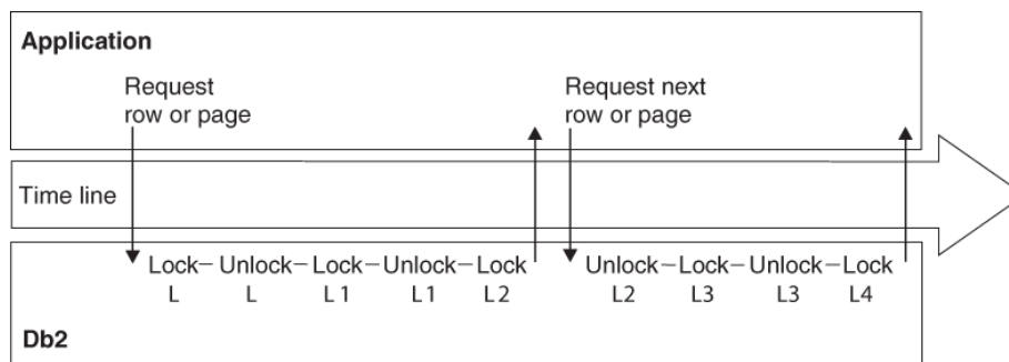
Figure 17. How an application that uses CS isolation with CURRENTDATA (YES) acquires locks
