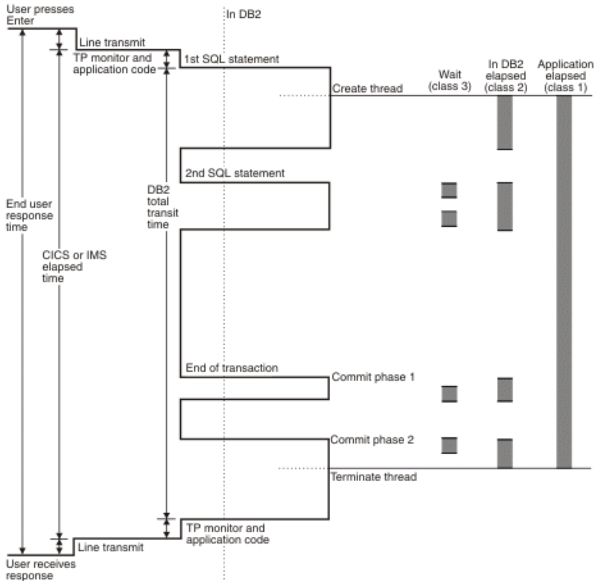
Figure 45. Transaction response times
