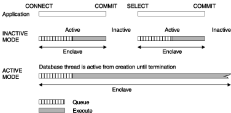
Figure 44. Contrasting ACTIVE MODE threads and POOLED MODE threads
