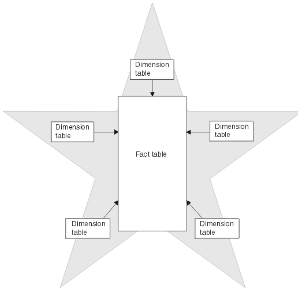
Figure 52. Star schema with a fact table and dimension tables
