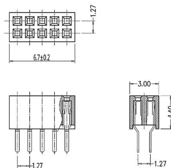
Figure 2-1 Mating terminals(for reference only)
