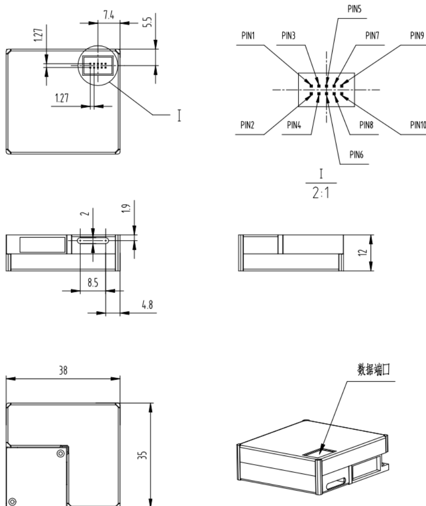
Figure 4-Dimension
