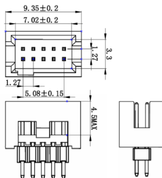
Figure 2-Terminal Model (PH=2x5x1.27mm)
