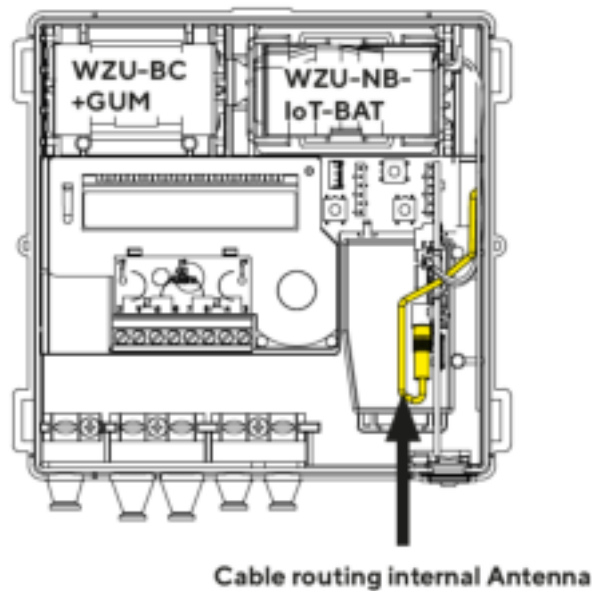
Figure 5: Cable routing internal antenna
