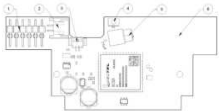
Figure 1: CMi6110 frontside
