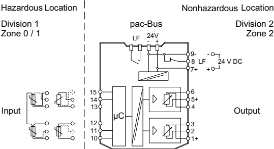
Connection Diagram 9180/20-77-11
