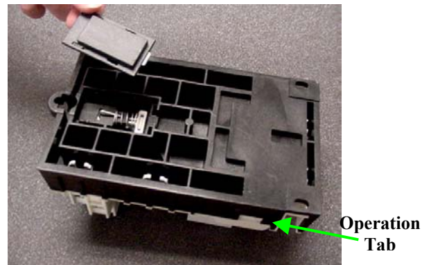
Figure 5 – Caution: Once latch cover has been installed, it may not be removed. Ensure latch is properly installed prior to installing the latch cover.
