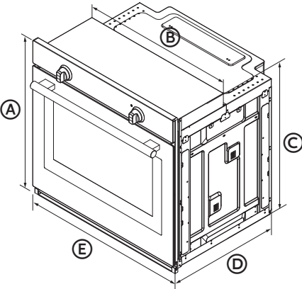
Single Oven
