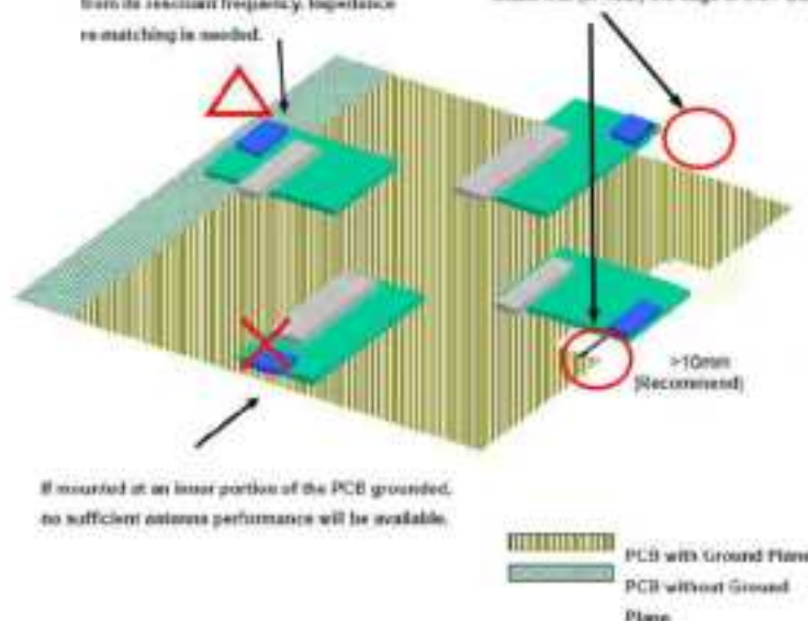
Figure 7 Module mounting position
