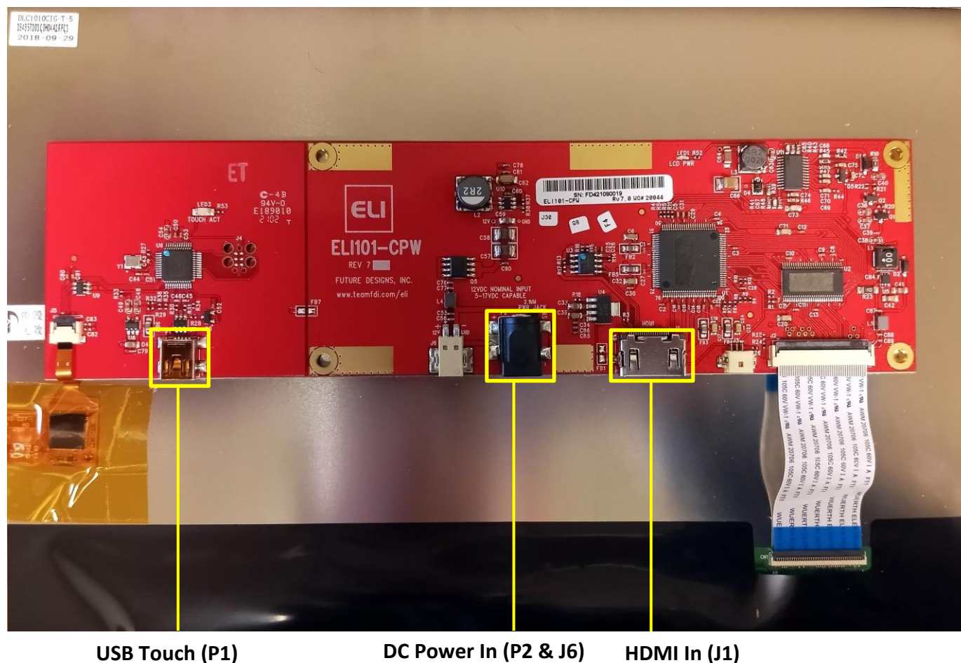
Figure 3. ELI101-CPW Connectors
