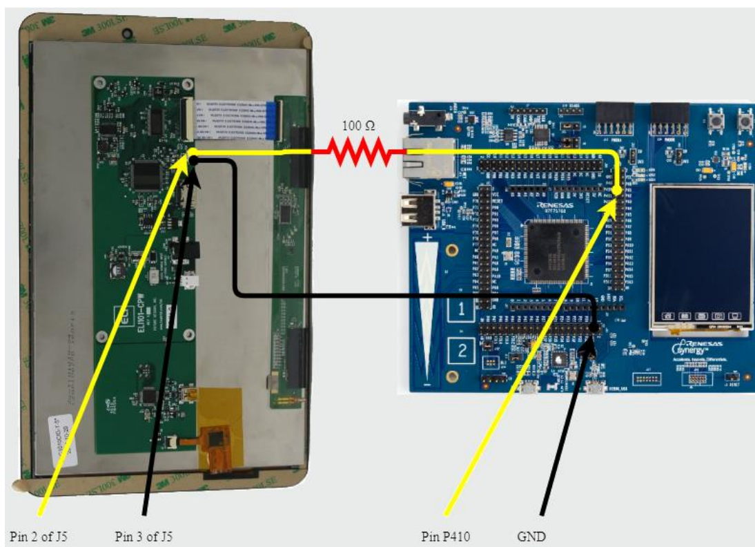
Figure 11. Renesas Synergy S7G2 Signal and Ground
