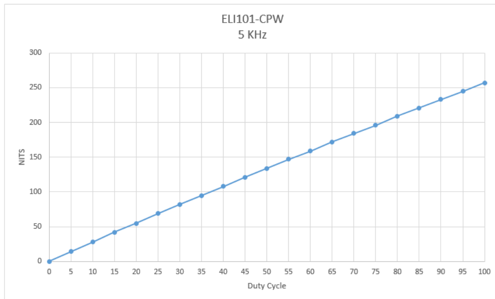
Figure 8. ELI101-CPW Backlight Curve in Nits
