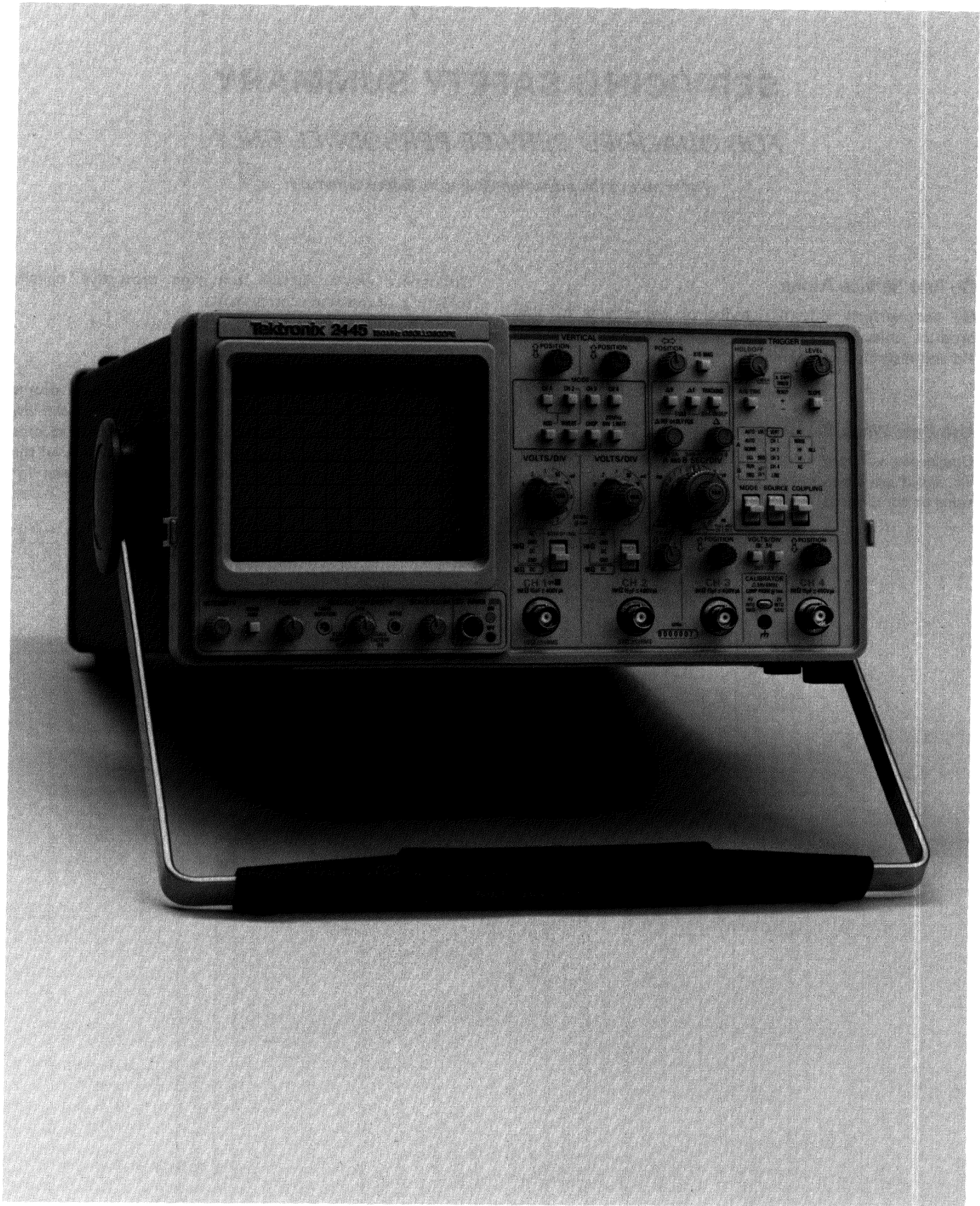
The 2445 Oscilloscope.
