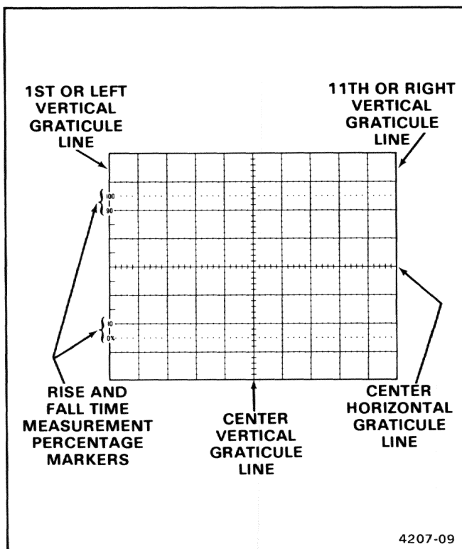
Figure 2-9. Graticule measurement markings.
