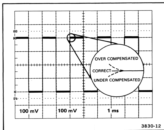
Figure 2-10. Probe low-frequency compensation.
