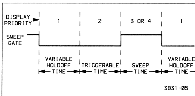
Figure 3-8. Readout display priorities.
