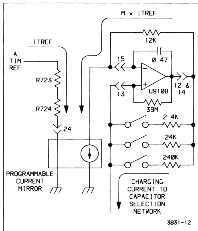
Figure 3-6. Sweep generator.
