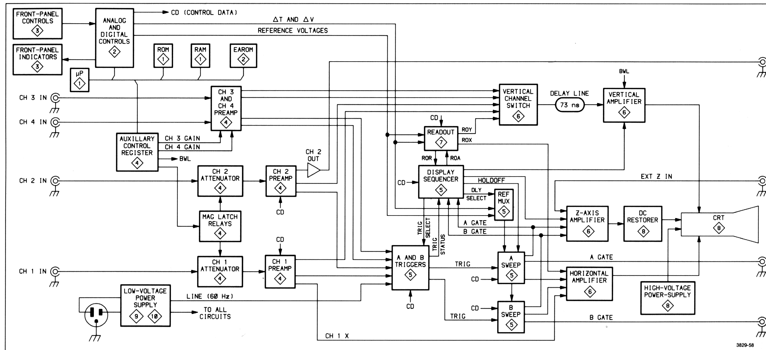
Figure 9-4. 2445 block diagram.
