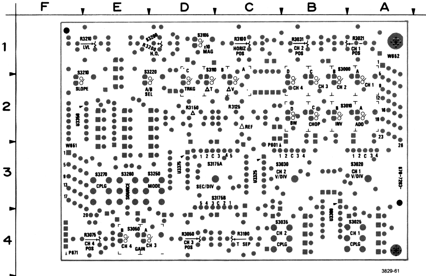
Figure 9-7. Circuit view of A6—Front Panel.
