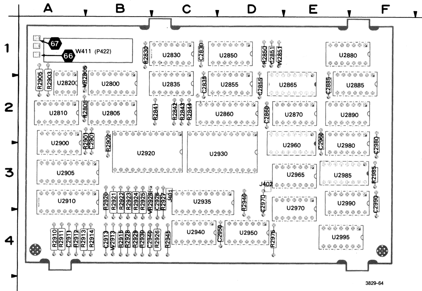
Figure 9-10. A4—Readout board.
