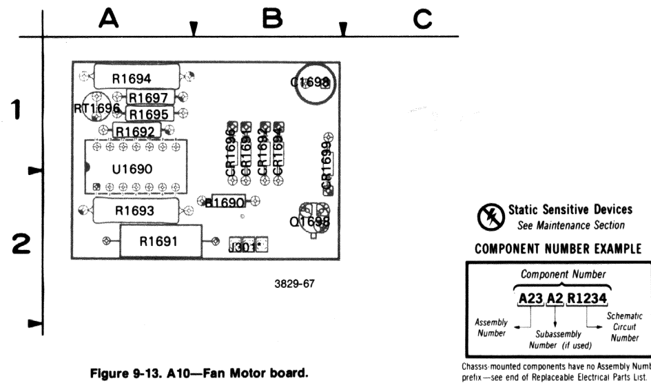
Figure 9-13. A10—Fan Motor board.
