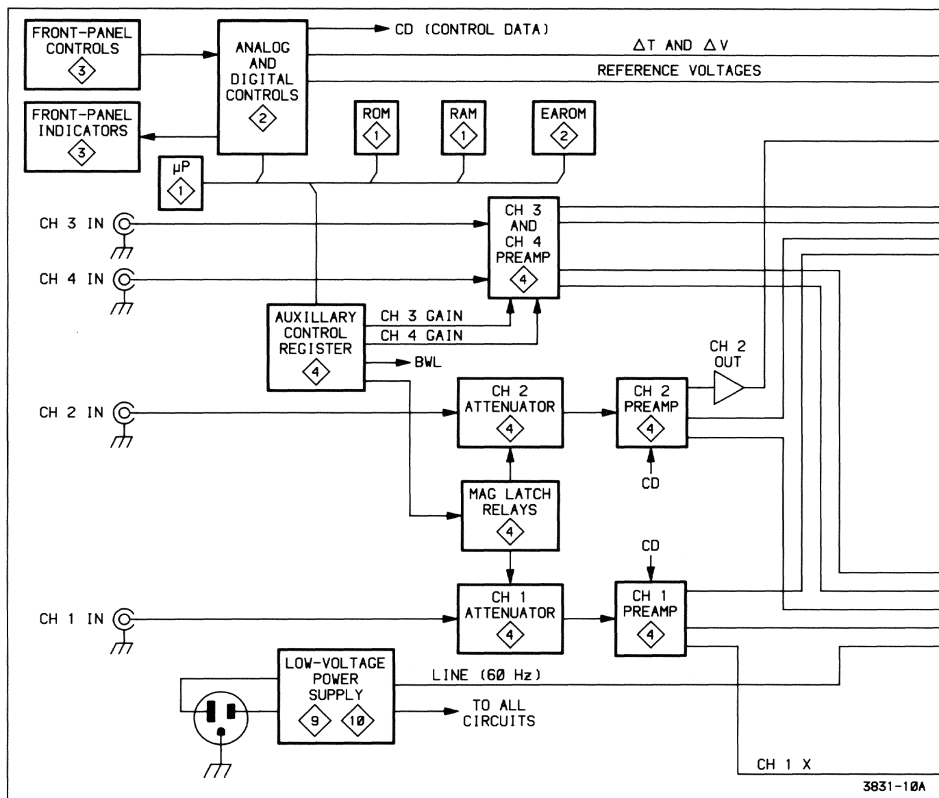
Figure 3-1. Block diagram.
