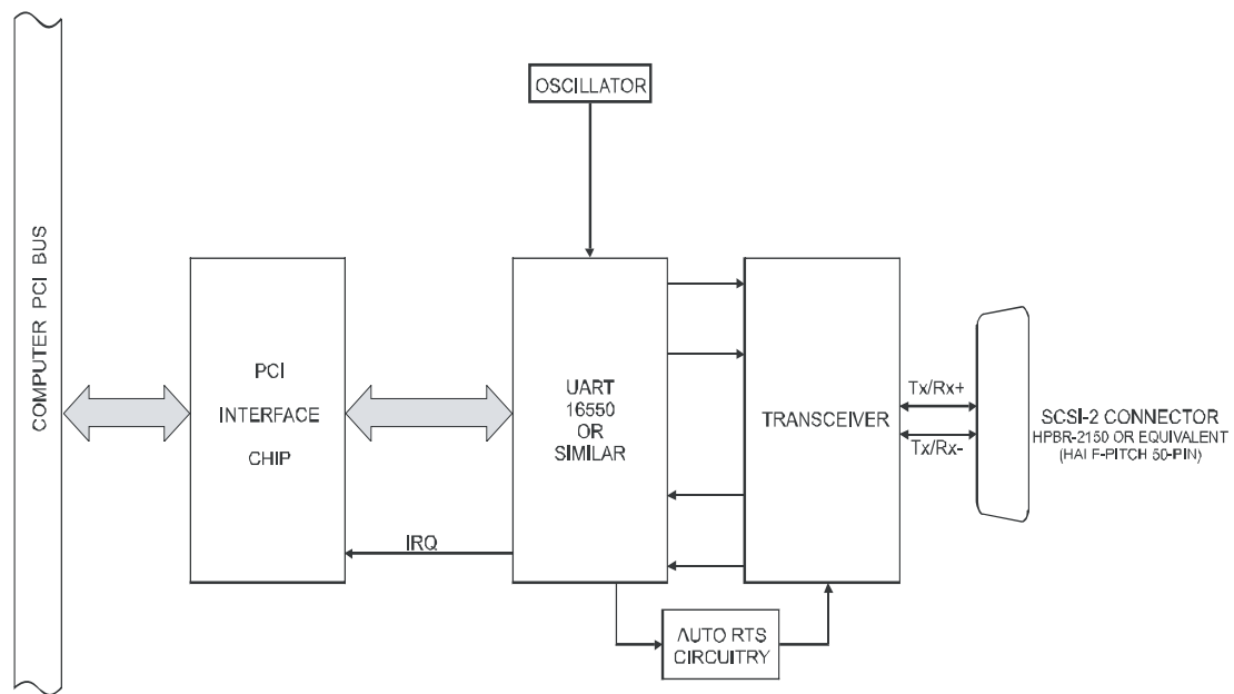
Figure 1-1: Block Diagram (only one serial channel shown)
